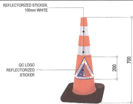
2 REFLECTORIZED TRAFFIC CONE SCALE : NOT TO SCALE
