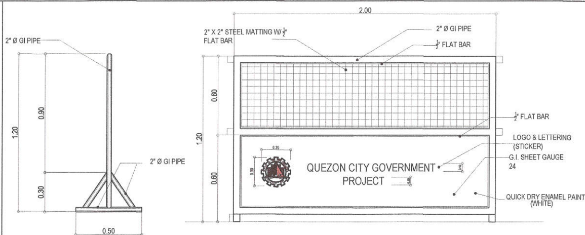
3 STEEL BARRICADE DETAIL SCALE : NOT TO SCALE
