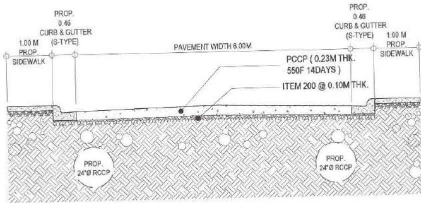
1 ROADWAY SECTION OF A
