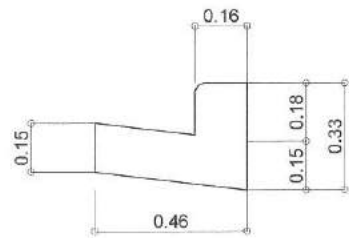
TYPE "A"
