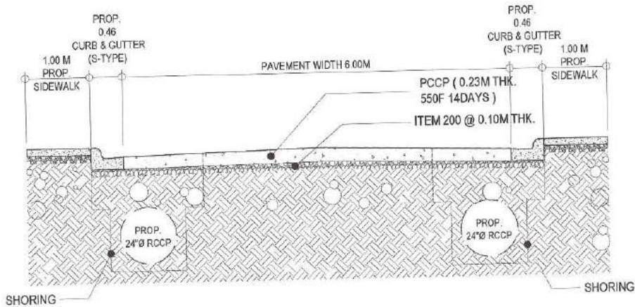
1 ROADWAY SECTION OF A
