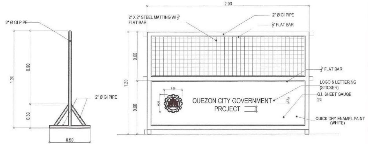
3 STEEL BARRICADE DETAIL
