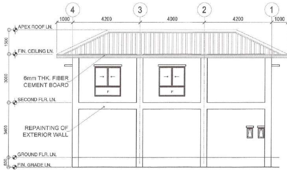
3 RIGHT SIDE VIEW
