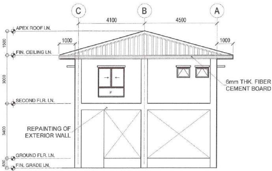
2 REAR VIEW
