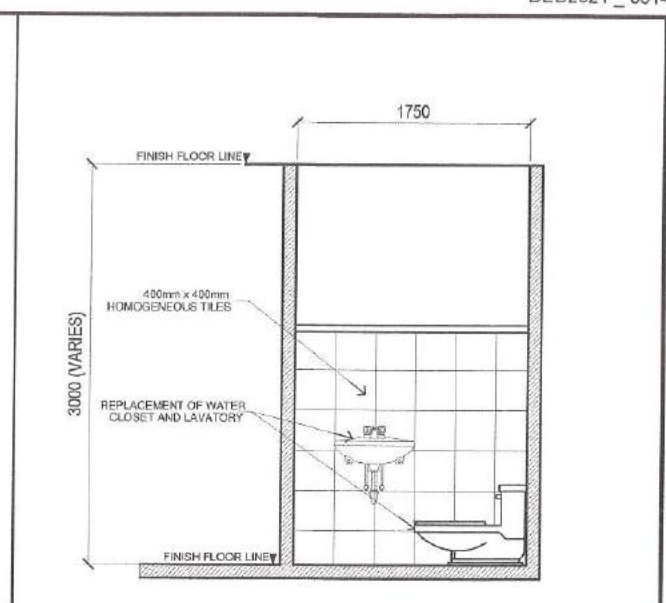
3 SECTION "B" SCALE: 1:40 METERS
