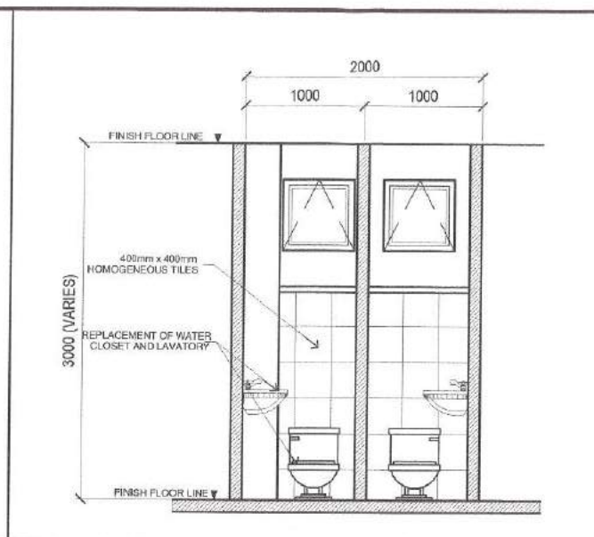
2 SECTION "A" SCALE: 1:40 METERS
