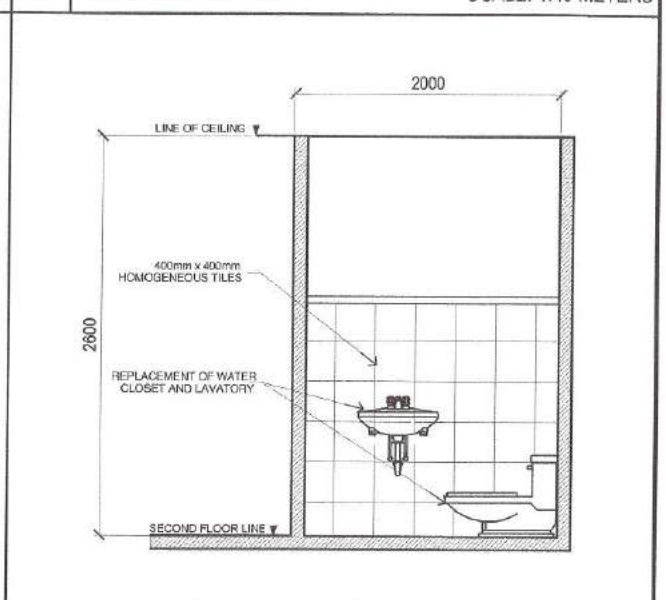
6 SECTION "D" SCALE: 1:40 METERS
