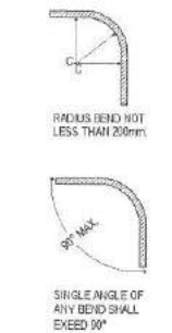
BENDING RADIUS DETAIL
