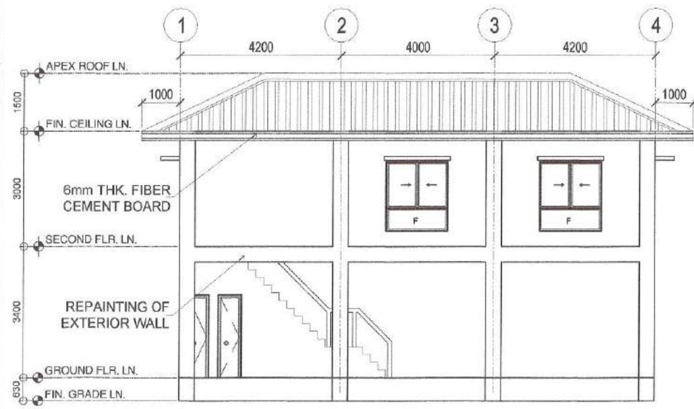
4 LEFT SIDE VIEW
