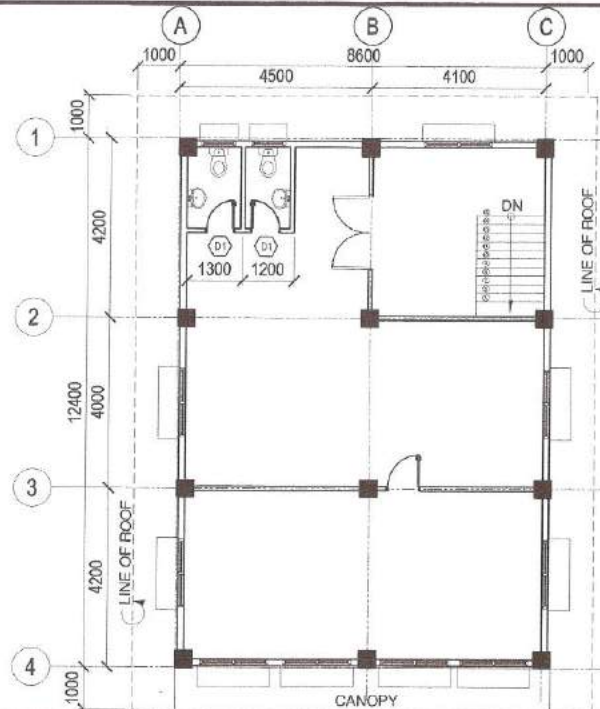
2 EXISTING 2/F PLAN SCALE: 1:125 METERS
