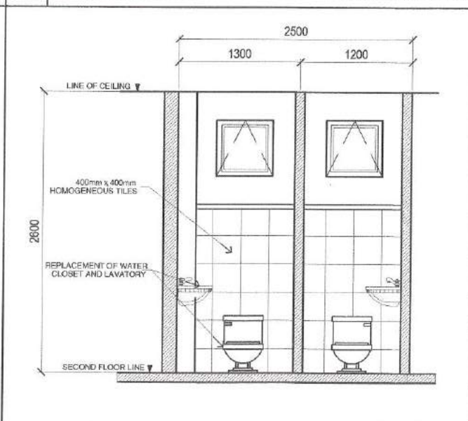
5 SECTION "C" SCALE: 1:40 METERS
