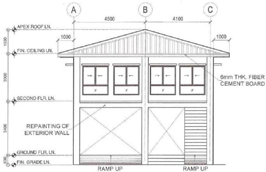
1 FRONT VIEW
