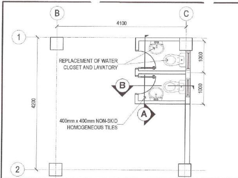
1 G/F TOILET BLOW-UP DETAILS SCALE: 1:50 METERS
