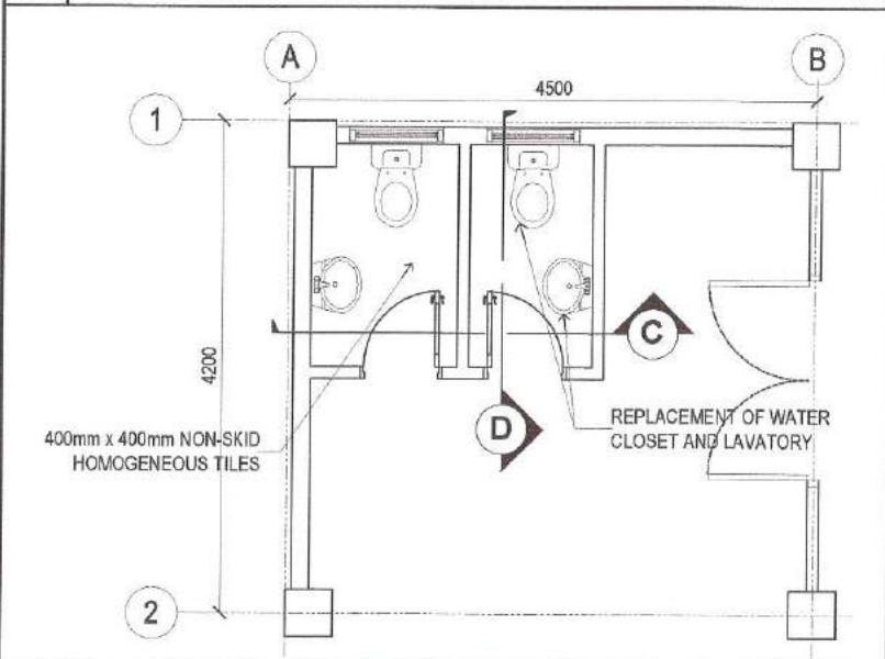
4 2/F TOILET BLOW-UP DETAILS SCALE: 1:50 METERS
