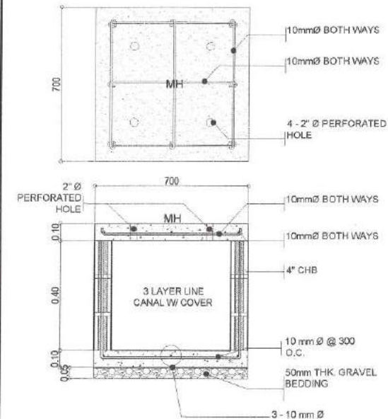
5 TYPICAL DETAIL FOR 3-LAYER LINED CANAL
