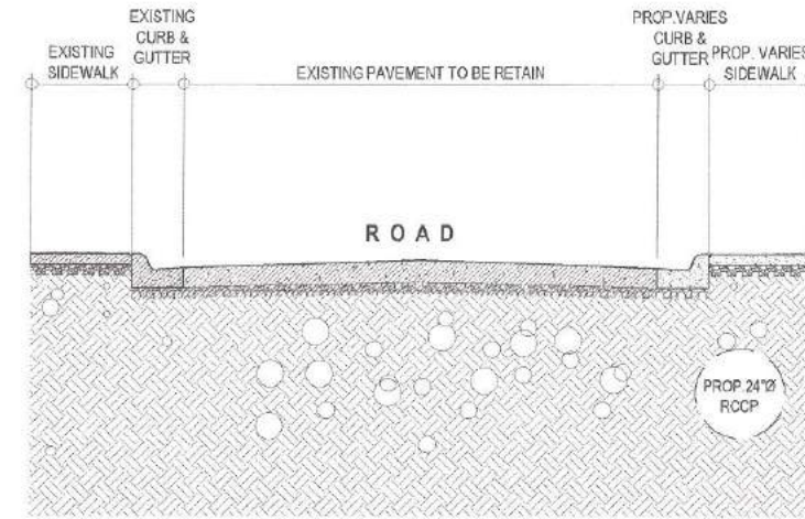
3 ROADWAY SECTION OF C
