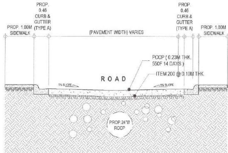
1 ROADWAY SECTION OF A
