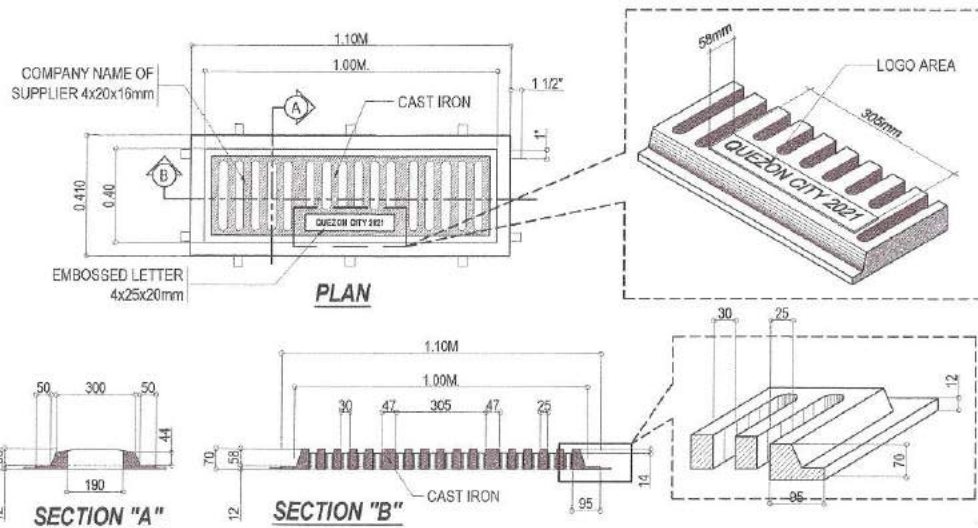
ELEVATION SECTION
