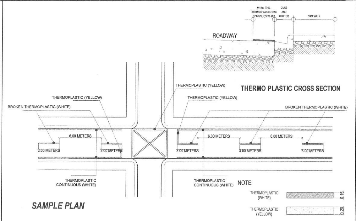
4 THERMO PLASTIC DETAIL SCALE: NTS
