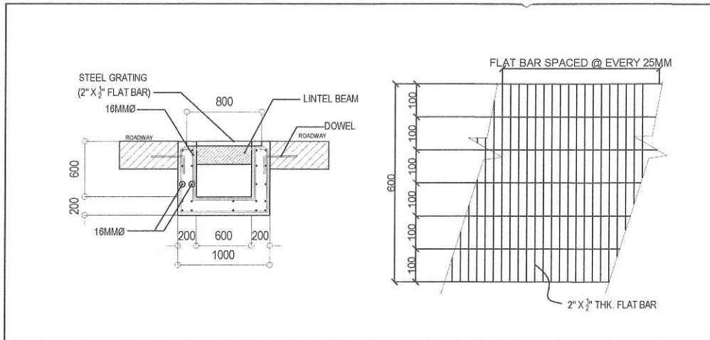
1 INTERCEPTOR DETAIL SCALE: NTS
