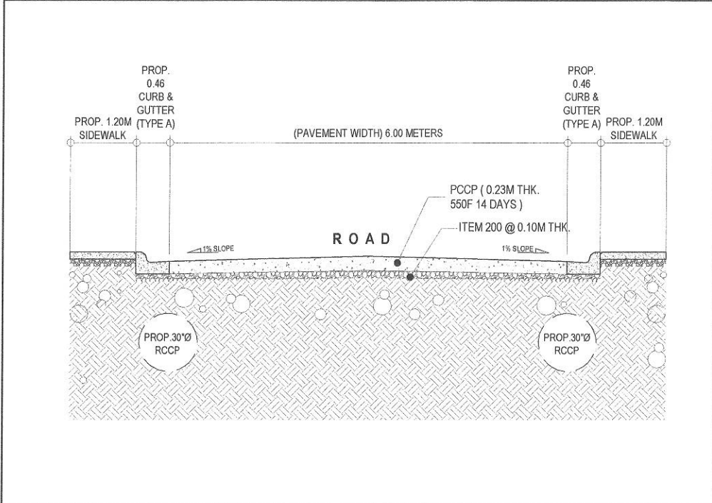
2 ROADWAY CROSS SECTION OF A SCALE: NTS
