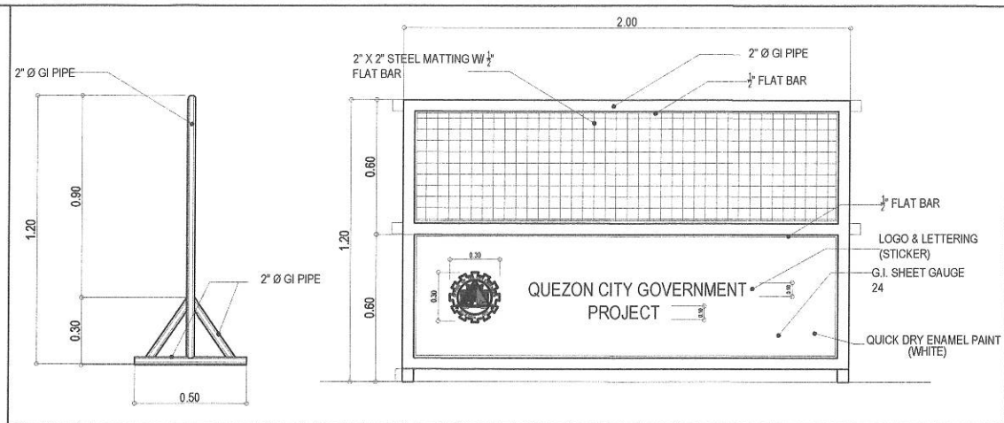
3 STEEL BARRICADE DETAIL SCALE: NTS
