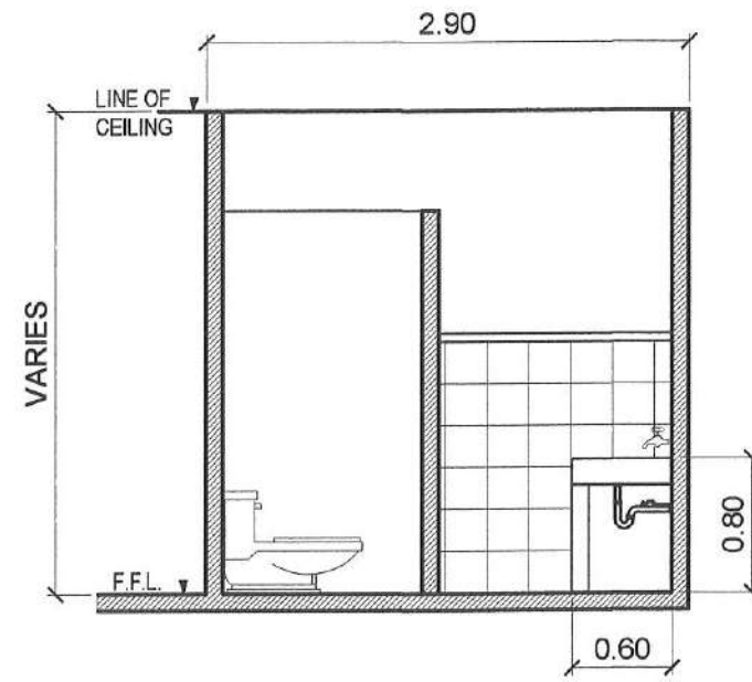
SECTION - B
