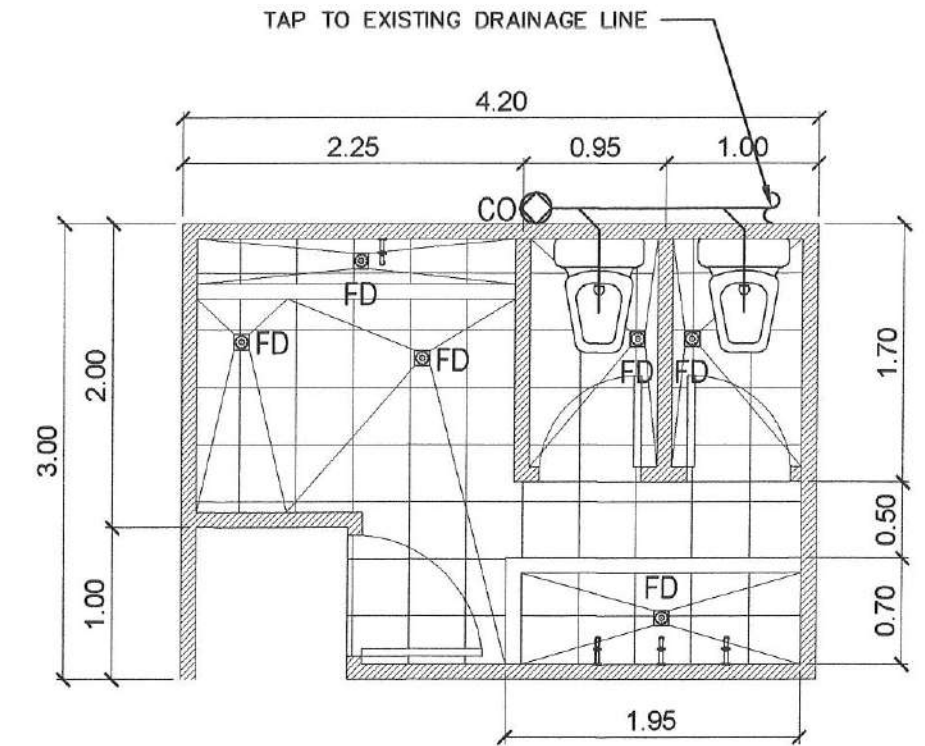
5 VARGAS BUILDING (2ND, 3RD & 4TH FLOOR MALE CR) SANITARY LAYOUT
