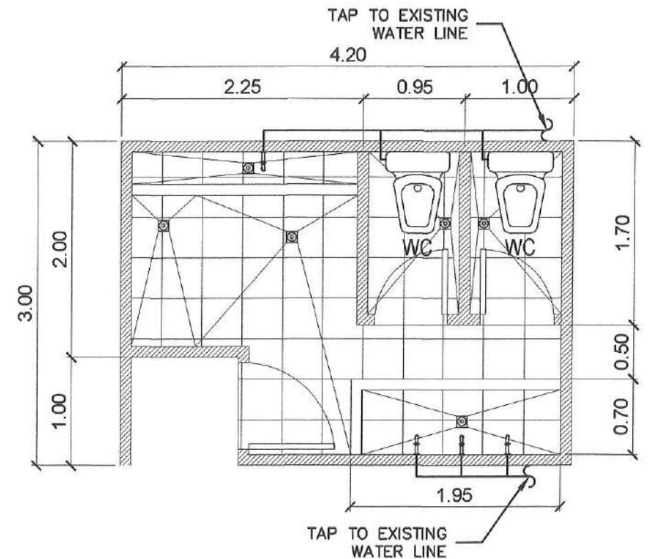
6 VARGAS BUILDING (2ND, 3RD & 4TH FLOOR MALE CR) WATER LINE LAYOUT
