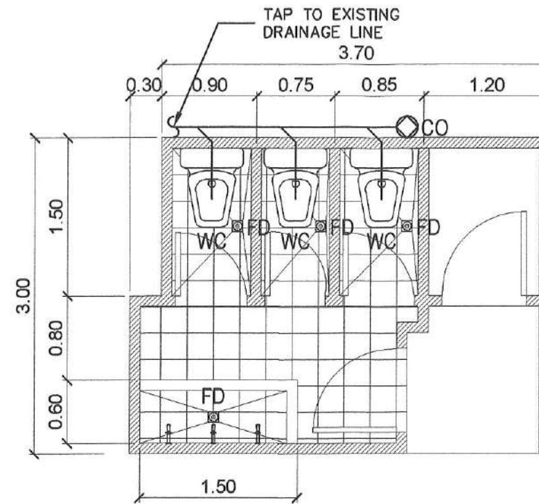
3 VARGAS BUILDING (2ND, 3RD & 4TH FLOOR FEMALE CR) SANITARY LAYOUT
