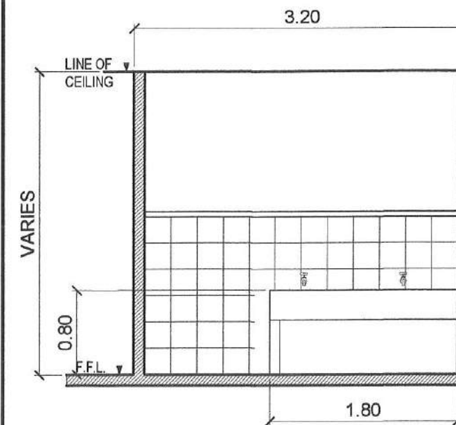
SECTION - A
