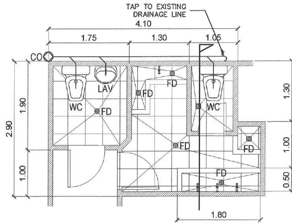
1 VARGAS BUILDING (GROUND FLOOR MALE CR) SANITARY LAYOUT
