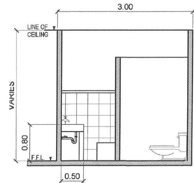
SECTION - B
