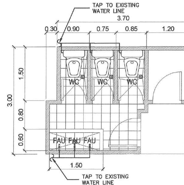
4 VARGAS BUILDING (2ND, 3RD & 4TH FLOOR FEMALE CR) WATER LINE LAYOUT
