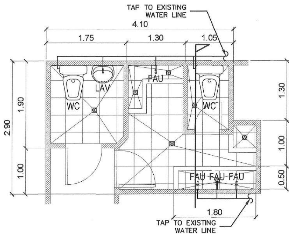
2 VARGAS BUILDING (GROUND FLOOR MALE CR) WATER LINE LAYOUT
