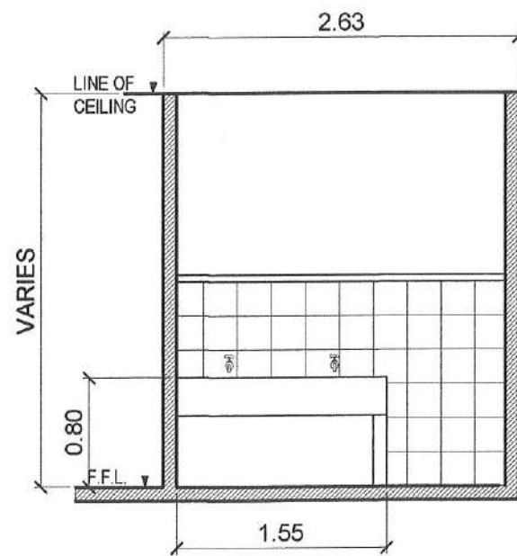
SECTION - A
