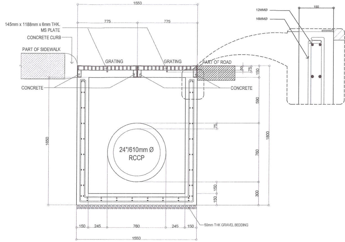
ELEVATION SECTION A-A
