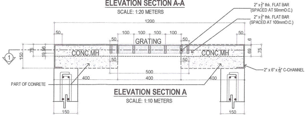
ELEVATION SECTION A-A
