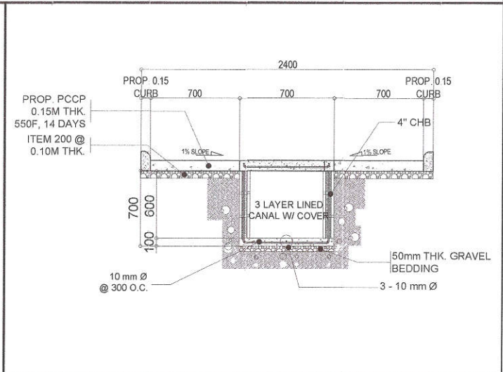
5 ROADWAY SECTION OF C SCALE : NOT TO SCALE
