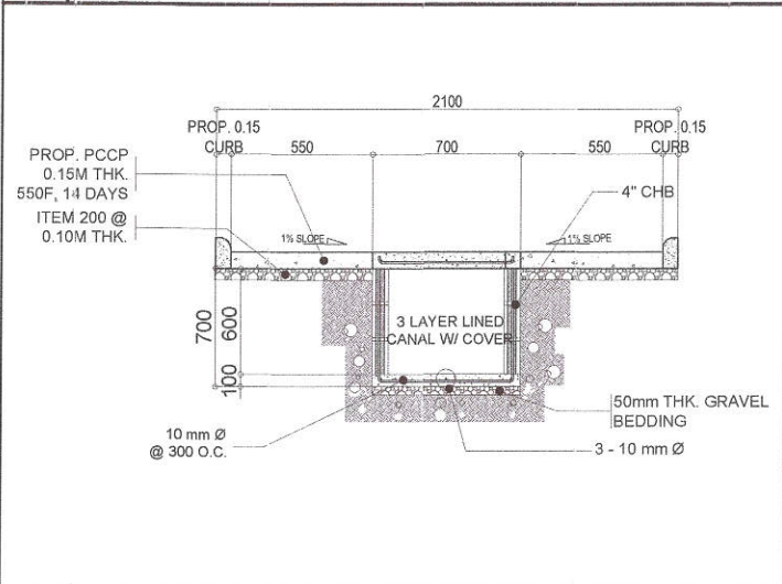
3 ROADWAY SECTION OF A SCALE : NOT TO SCALE
