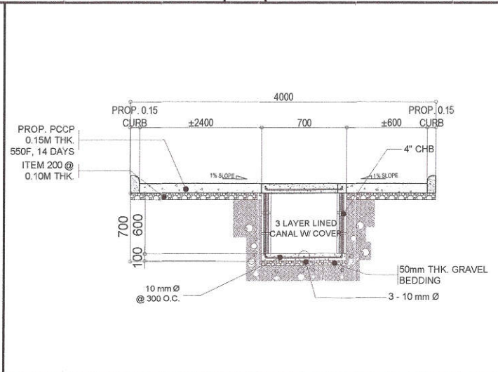
4 ROADWAY SECTION OF B SCALE : NOT TO SCALE
