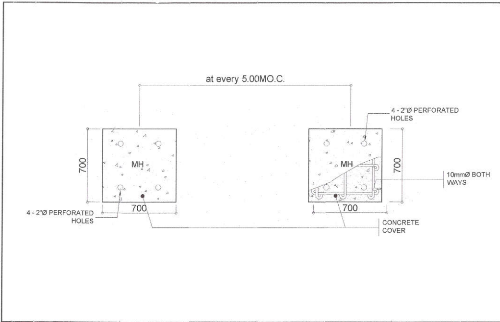
1 3 LAYER LINED CANAL CONCRETE COVER DETAIL
