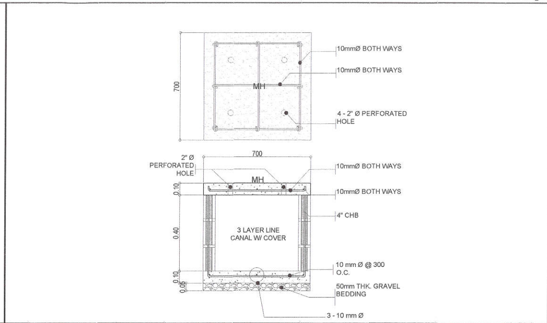
2 TYPICAL DETAIL 3-LAYER LINED CANAL SCALE : NOT TO SCALE
