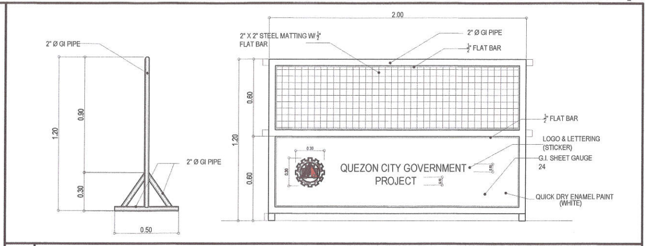
2 STEEL BARRICADE DETAIL SCALE: NTS
