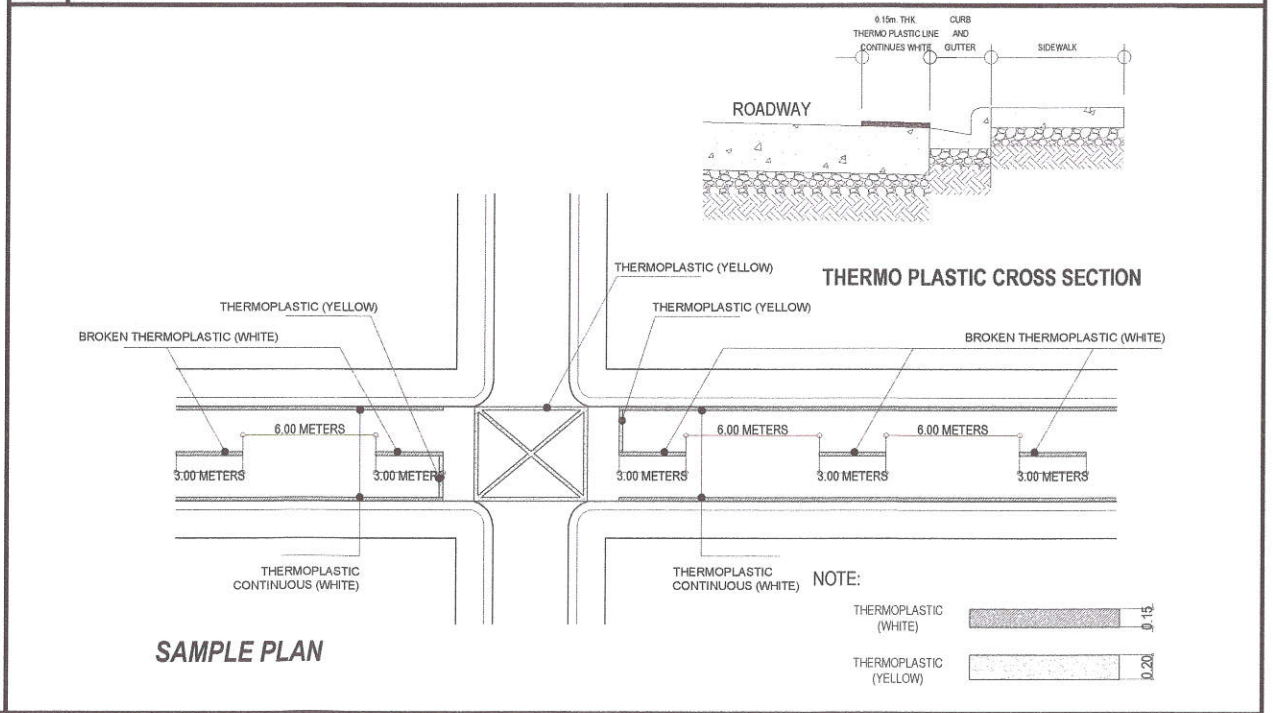
3 THERMO PLASTIC DETAIL SCALE: NTS
