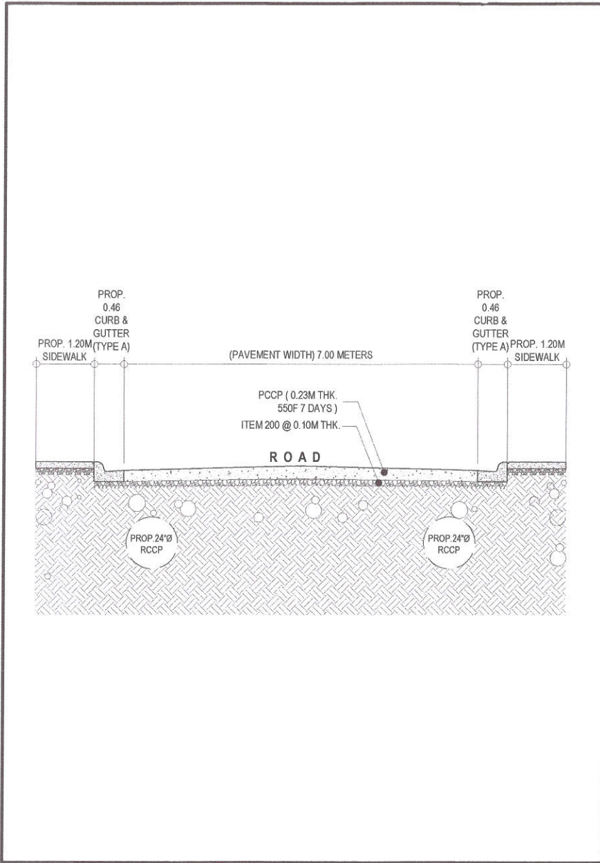
1 ROADWAY CROSS SECTION OF A SCALE: NTS
