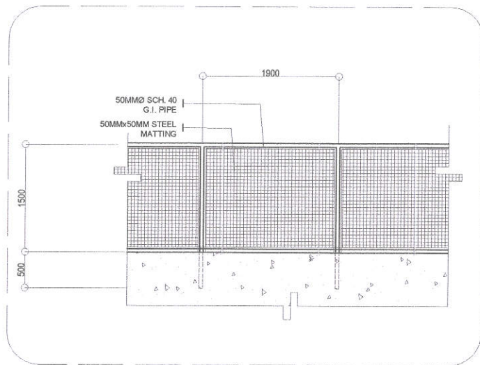
STEEL FENCE DETAIL
