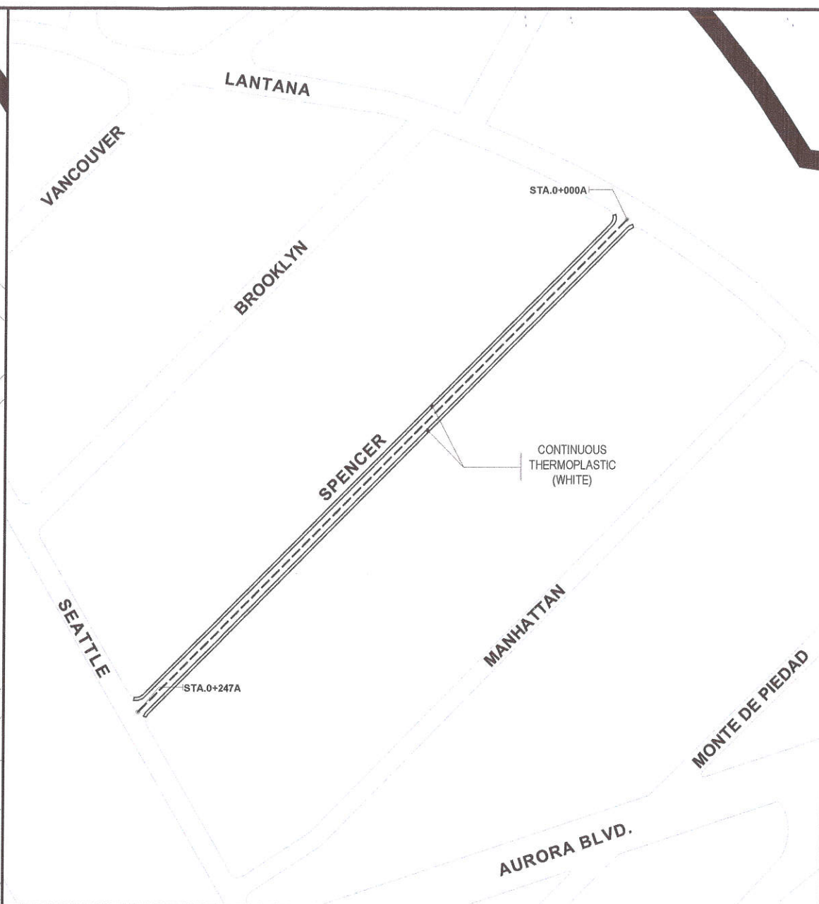
2 ROADWAY PLAN WITH THERMO PLASTIC LANE MARKING OF SPENCER STREET SCALE : NOT TO SCALE
