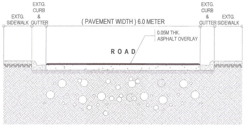
1 ROADWAY CROSS SECTION OF A
