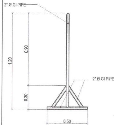
3 STEEL BARRICADE DETAIL
