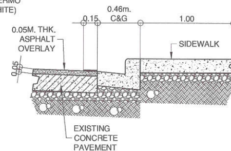
THERMO PLASTIC SECTION
