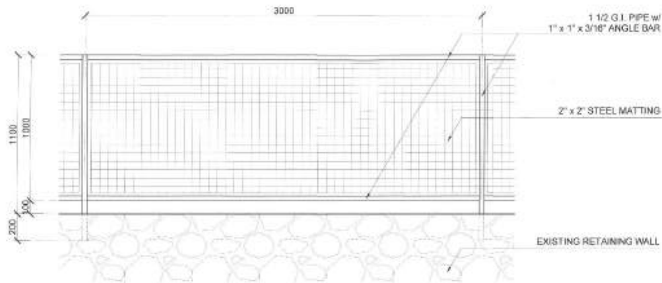
1 SECURITY FENCE DETAIL SCALE 1:20 MTS.
