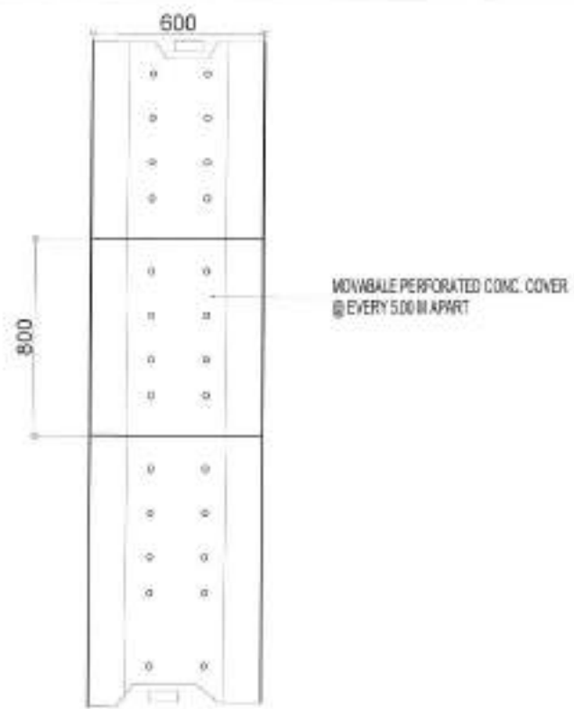
PLAN
