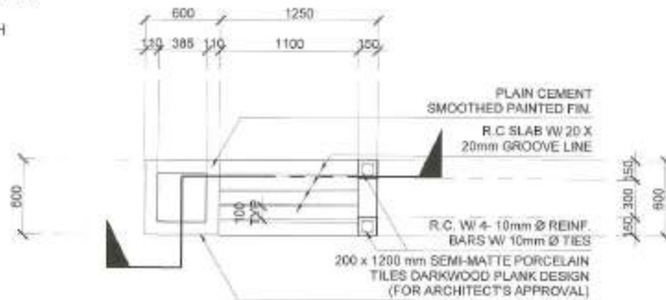
PLAN
