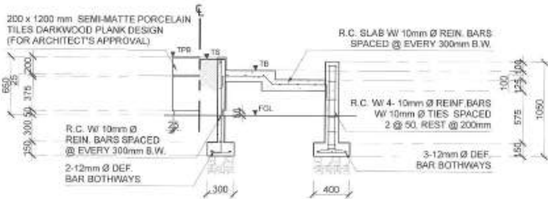
ELEVATION-A/ SECTION-A
