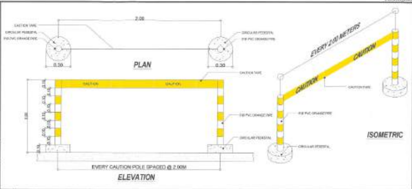
4 SAFETY STRUCTURE SCALE : NTS
