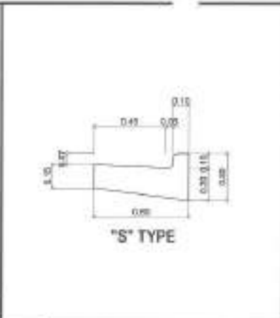
2 THERMO PLASTIC DETAIL NTS
