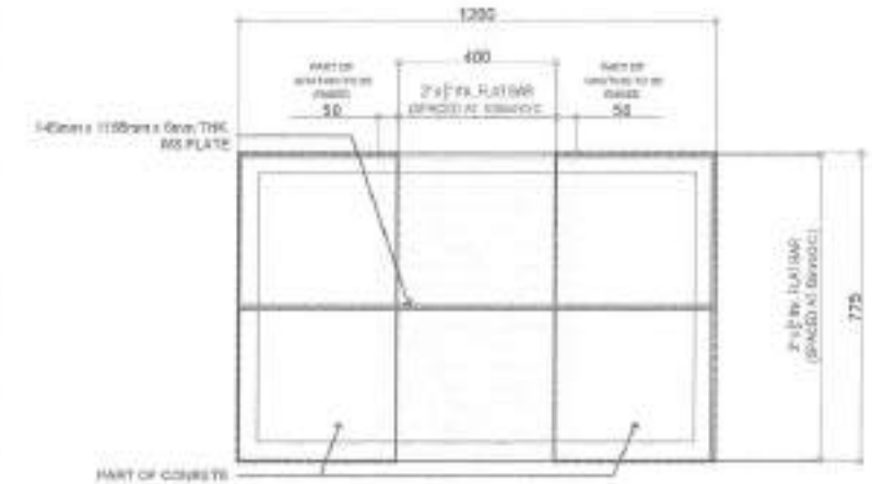
VIEW FOR SECTION 1 SCALE: 1:15 METERS
