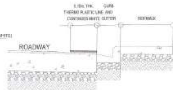
THERMO PLASTIC CROSS SECTION
