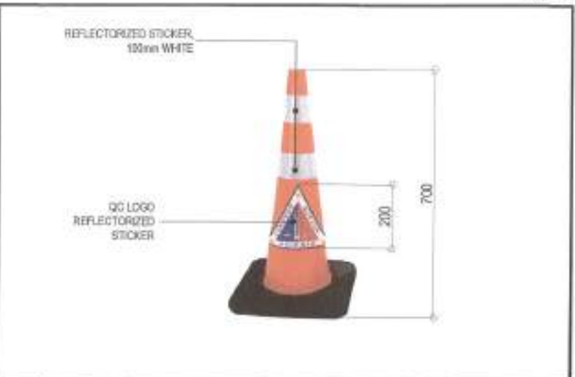
3 REFLECTORIZED TRAFFIC CONE NTS
