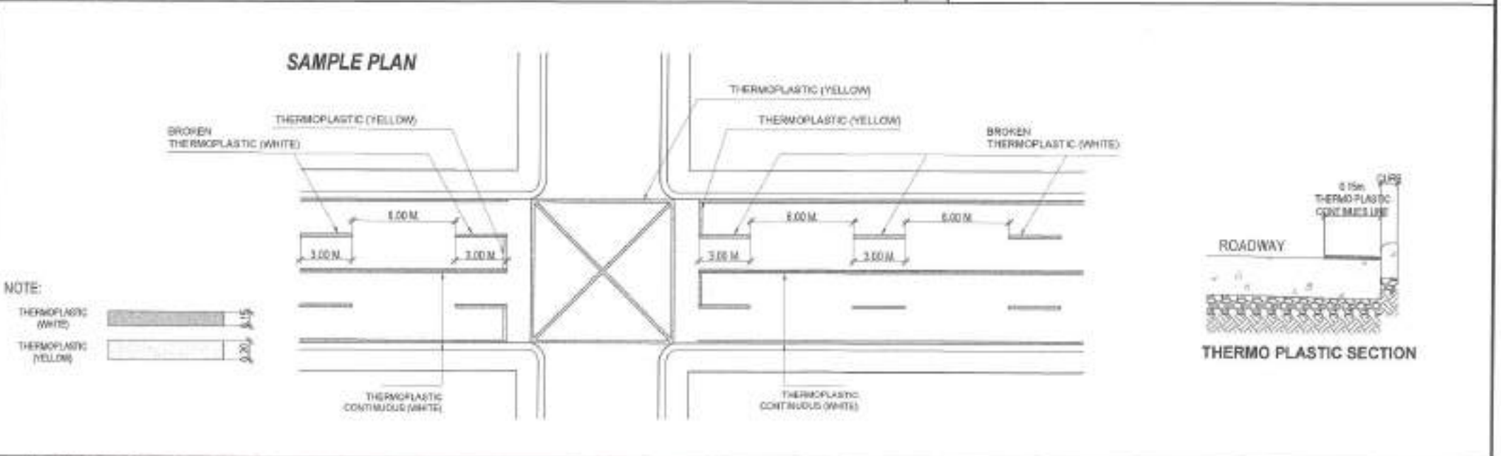
2 THERMO PLASTIC LANE MARKING DETAIL (4 LANES) SCALE: NOT TO SCALE
