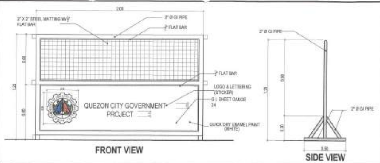
1 STEEL BARRICADE DETAIL SCALE: NOT TO SCALE
