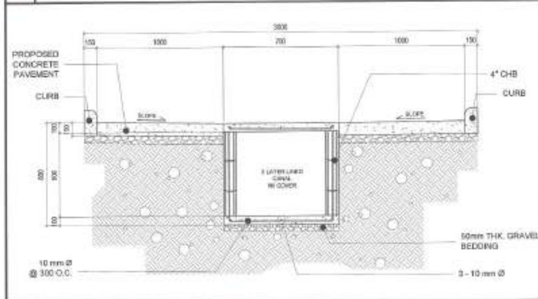
2 CROSS SECTION OF B SCALE: NOT TO SCALE
