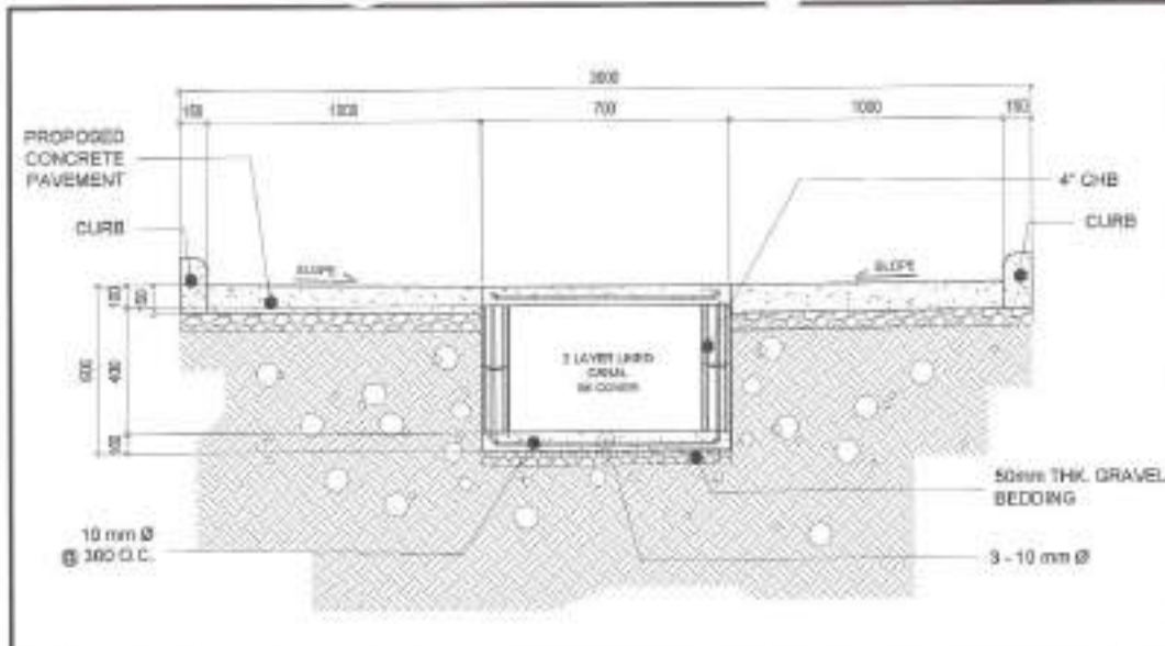
1 CROSS SECTION OF A SCALE: NOT TO SCALE
