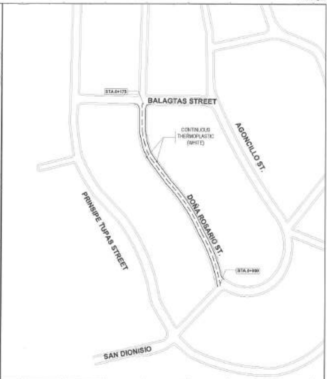
2 ROADWAY PLAN WITH THERMO PLASTIC LANE MARKING OF DOÑA ROSARIO STREET
