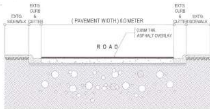
1 ROADWAY CROSS SECTION
