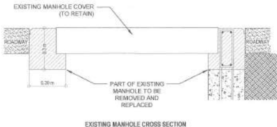
EXISTING MANHOLE CROSS SECTION
