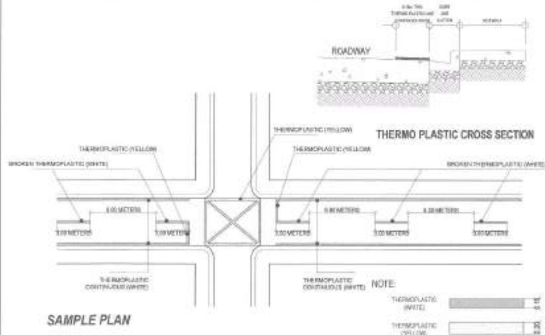
4 THERMO PLASTIC DETAIL
