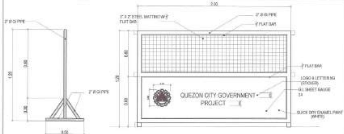
2 STEEL BARRICADE DETAIL
