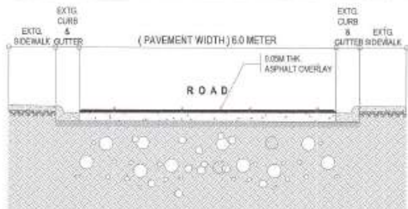
1 ROADWAY CROSS SECTION
