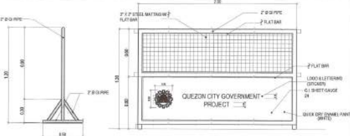
2 STEEL BARRICADE DETAIL
