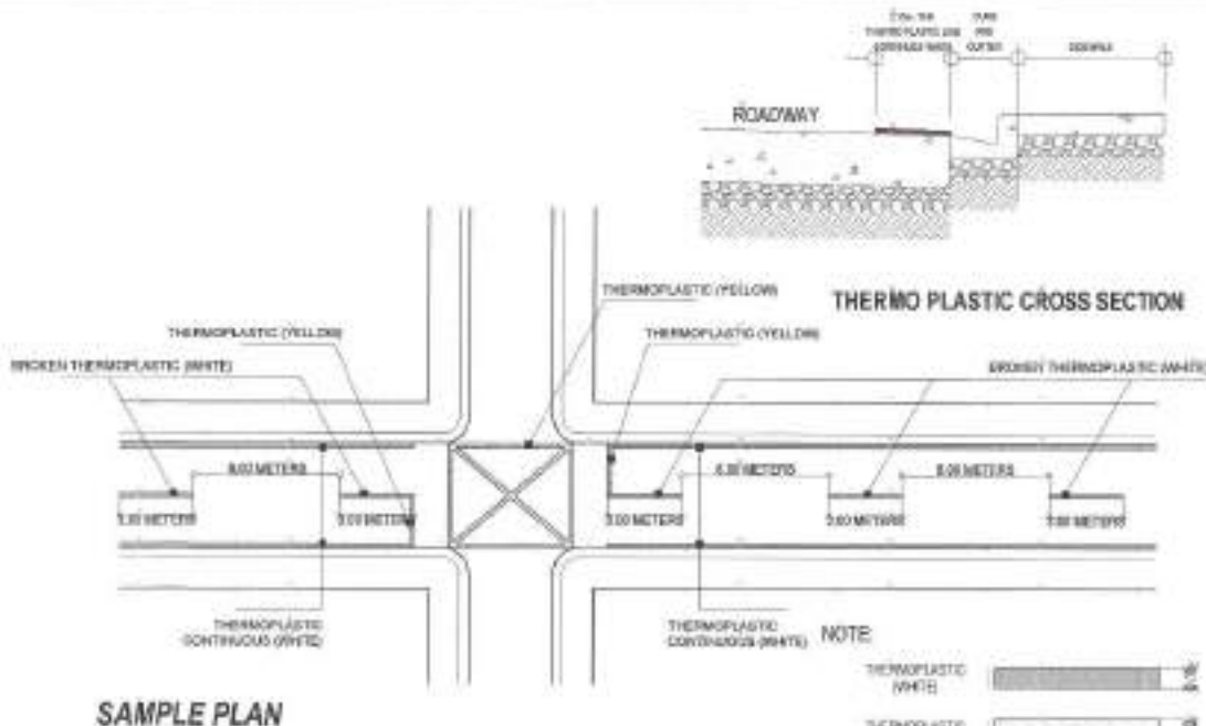
4 THERMO PLASTIC DETAIL
