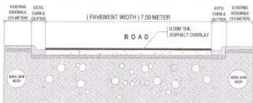
2 ROADWAY CROSS SECTION OF B SCALE : NOT TO SCALE
