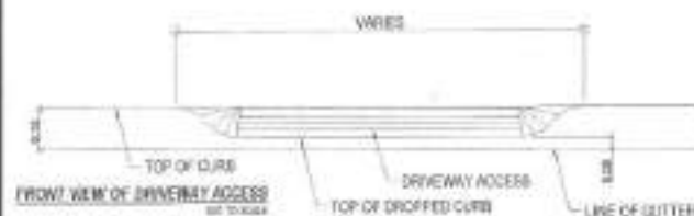
6 TYPICAL DRIVEWAY ACCESS DETAIL
