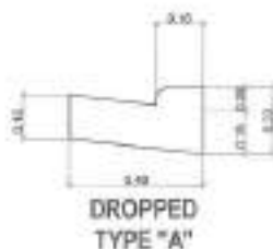
4 TYPICAL DROPPED CONCRETE CURB DETAIL
