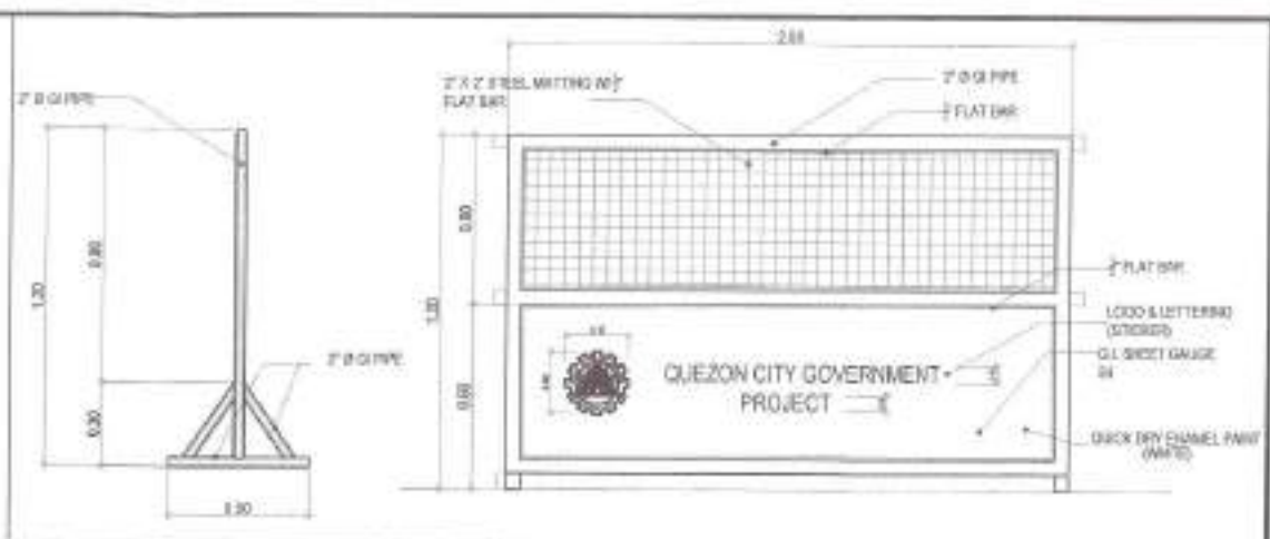
2 STEEL BARRICADE DETAIL SCALE: NOT TO SCALE
