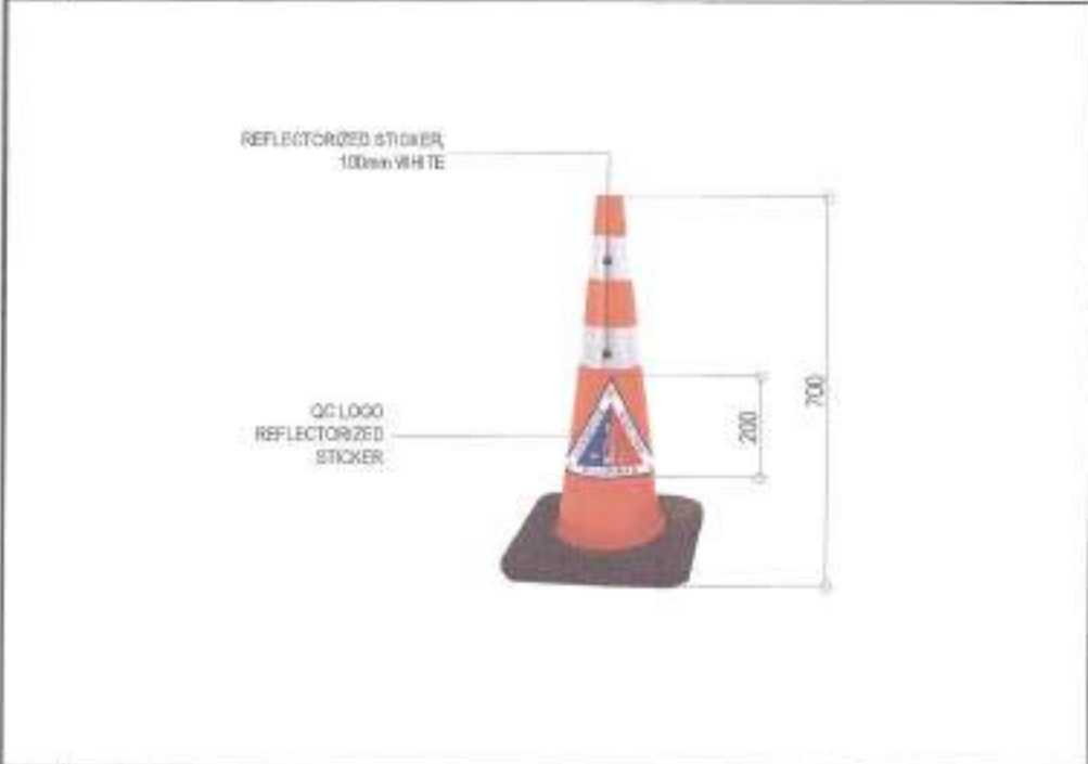
3 REFLECTORIZED TRAFFIC CONE SCALE: NOT TO SCALE
