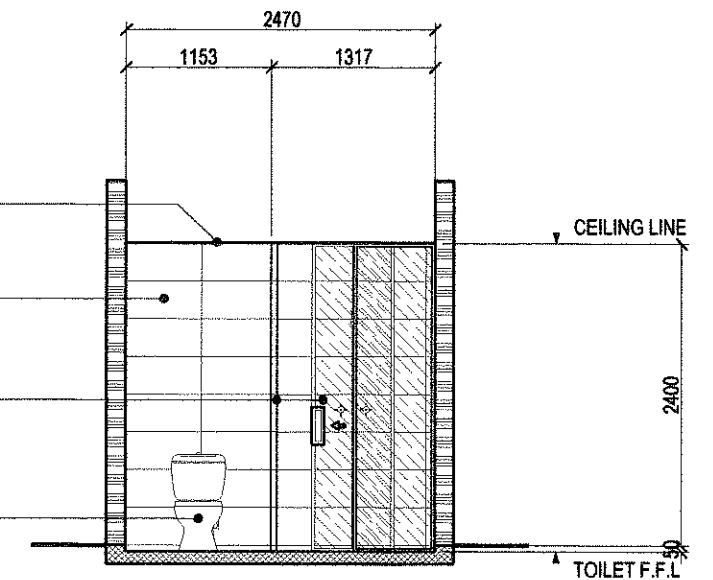
SECTION THRU 'C'
