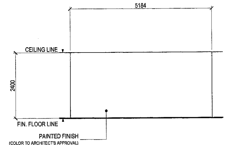
ELEVATION "D" / "E"
