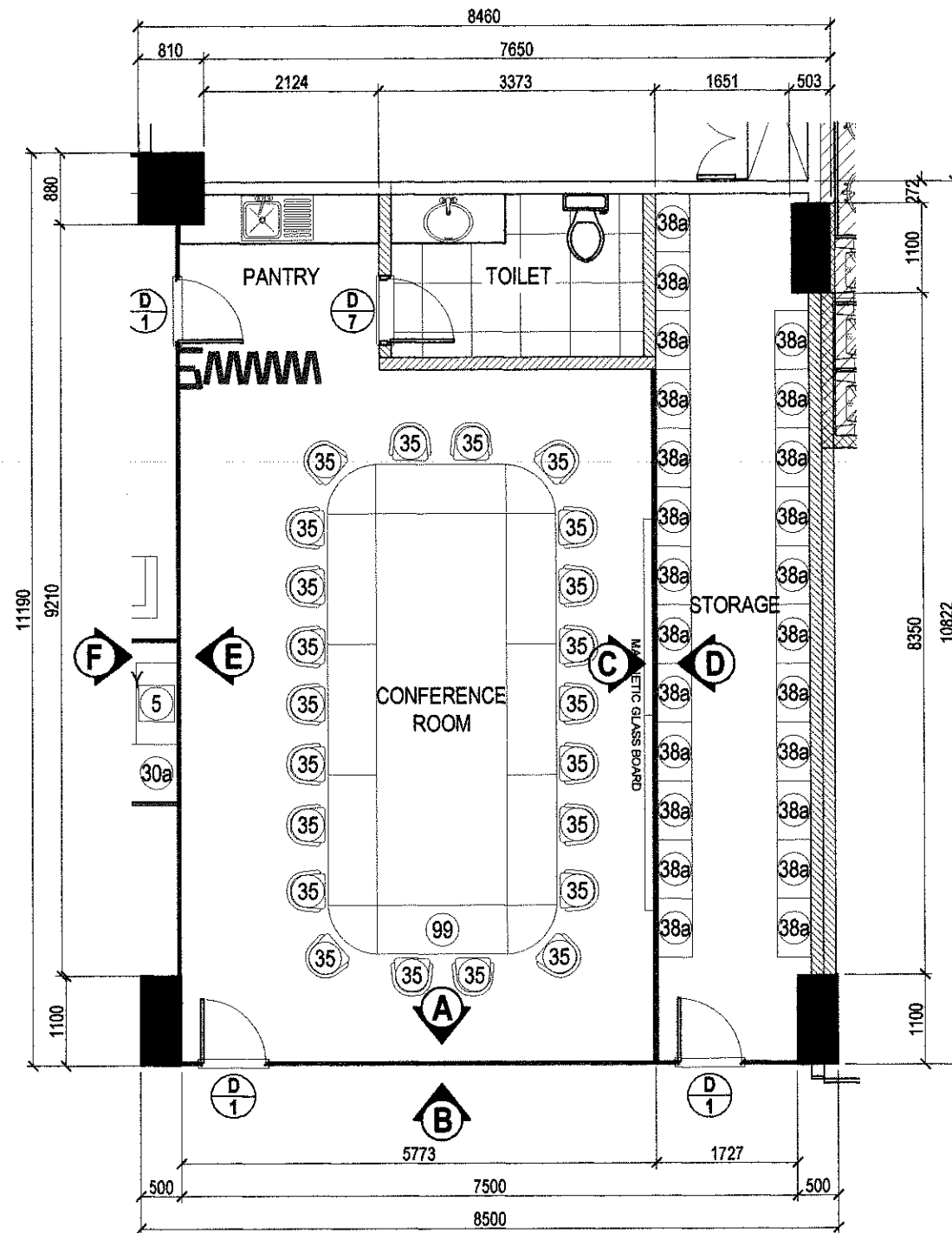
BLOW - UP PLAN
