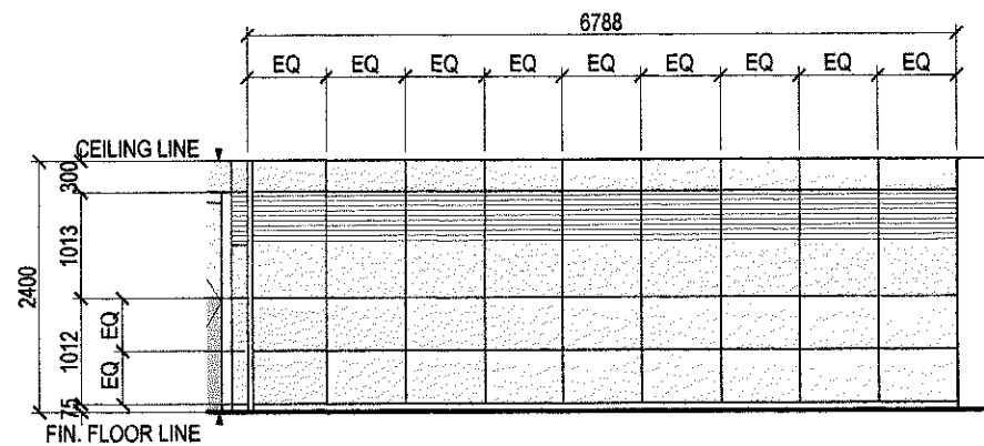
ELEVATION 'A'
