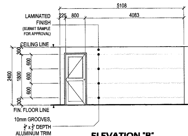
ELEVATION "B"
