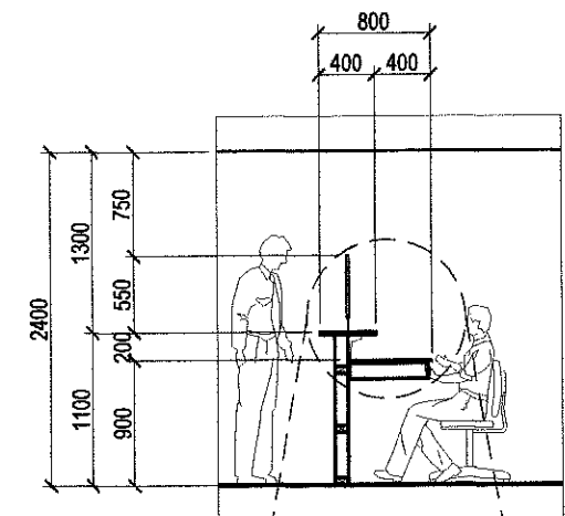
SECTION THRU 'D'
