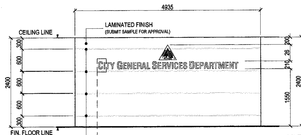
ELEVATION 'A'
