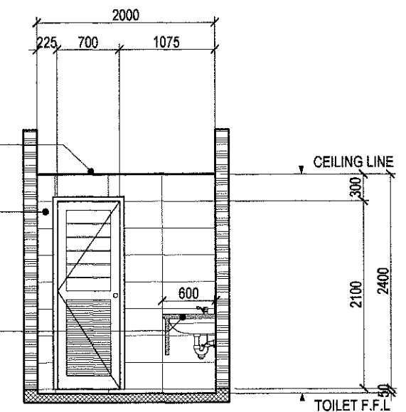
SECTION THRU 'D'
