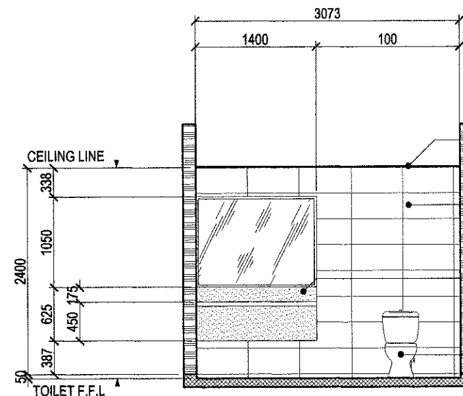
SECTION THRU 'A'
