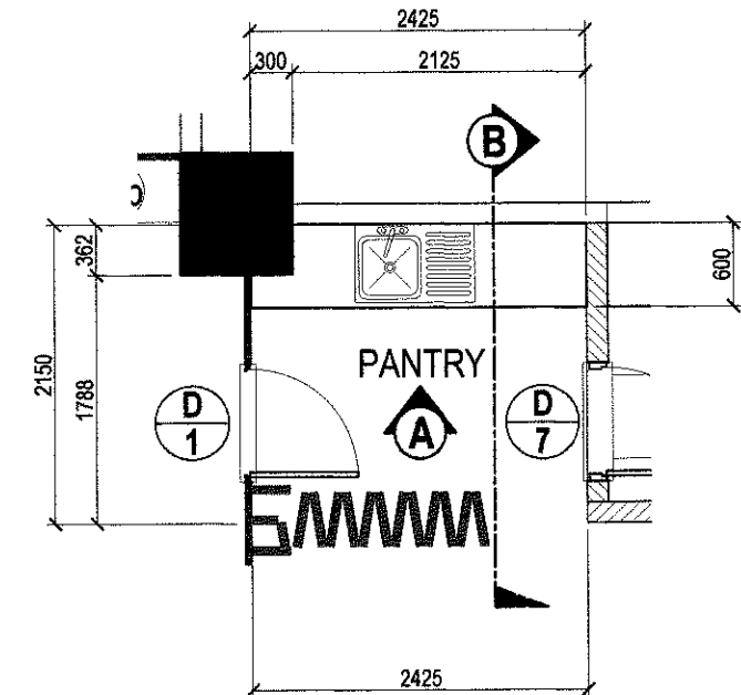
BLOW - UP PLAN
