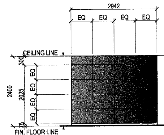
ELEVATION "B"
