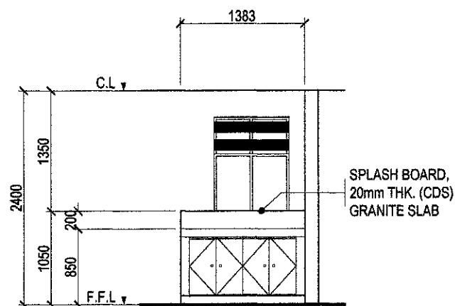
SECTION THRU 'A'
