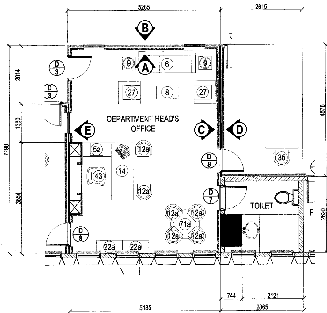
BLOW - UP PLAN
