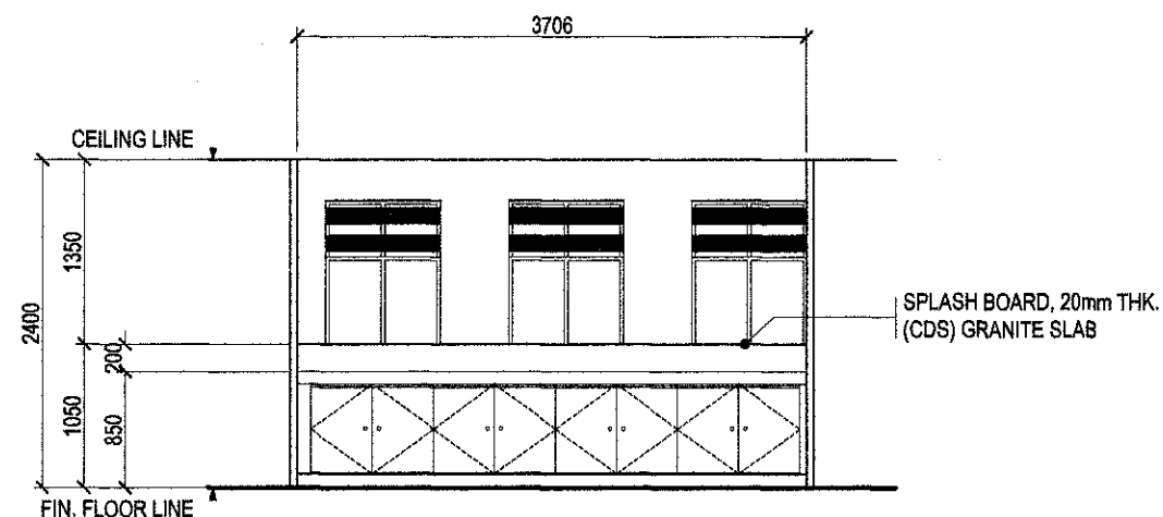
SECTION THRU 'A'
