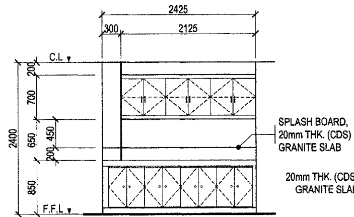
ELEVATION 'A'
