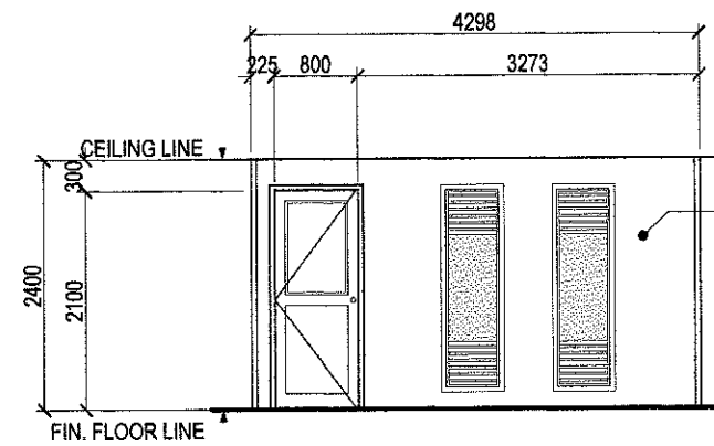
ELEVATION 'A'
