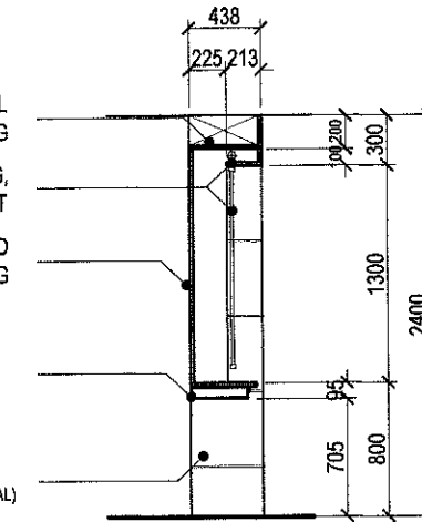
SECTION THRU 'A'
