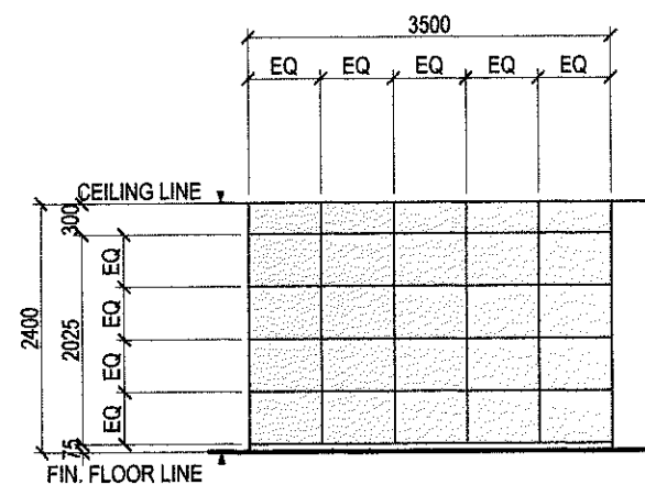
ELEVATION 'A'
