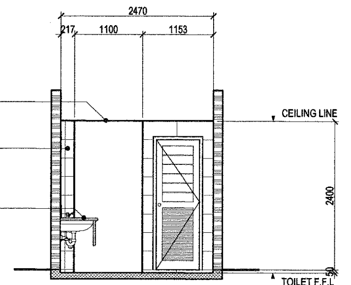
SECTION THRU 'D'
