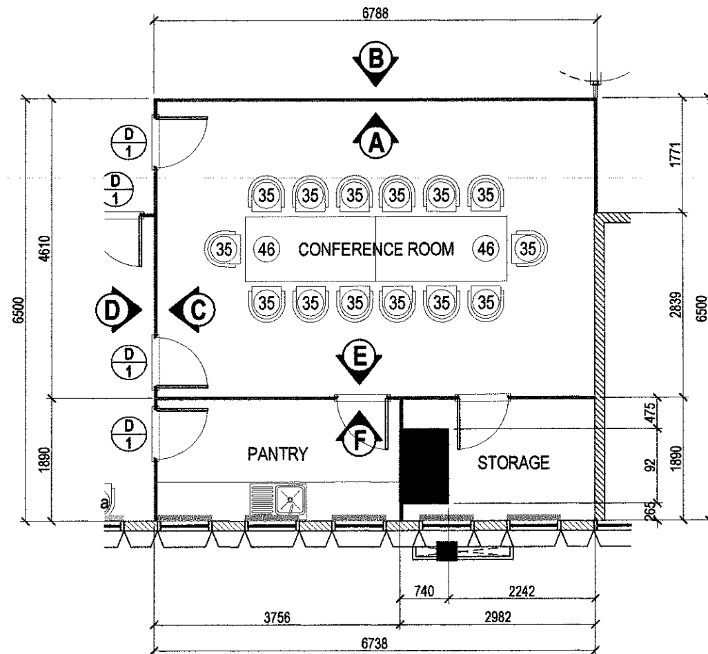
BLOW - UP PLAN
