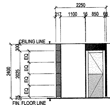
ELEVATION "D"
