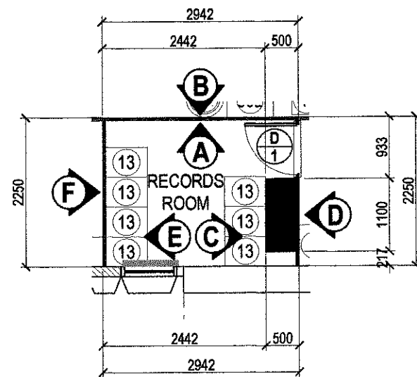
BLOW - UP PLAN
