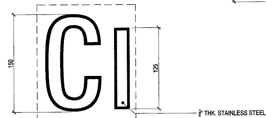
OFFICE SIGNAGE DETAIL
