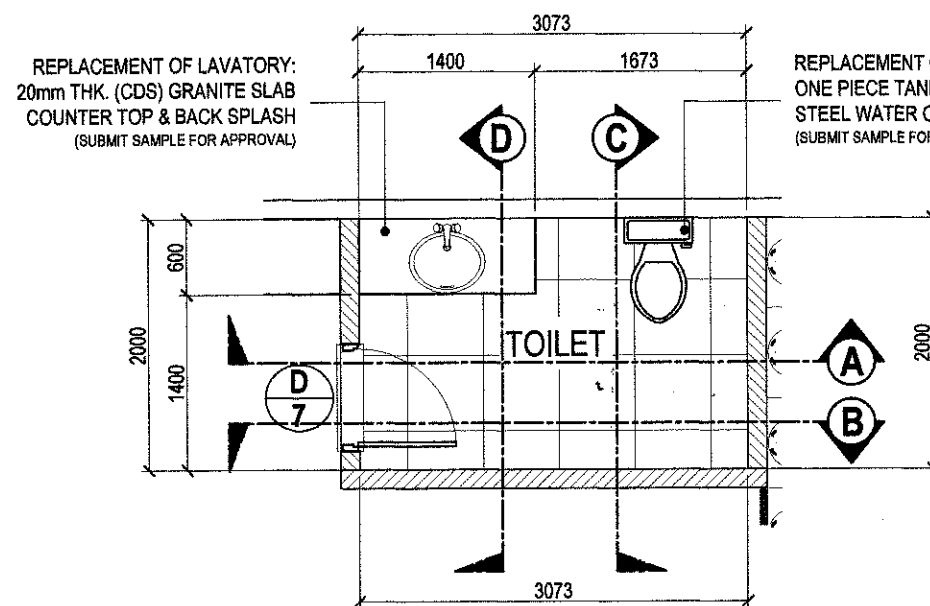
BLOW - UP PLAN
