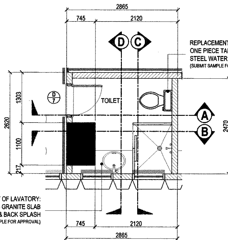
BLOW - UP PLAN
