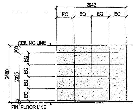
ELEVATION "A"
