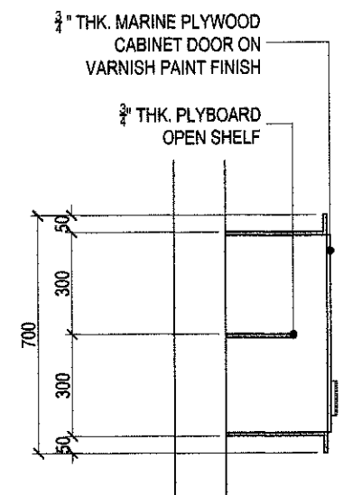
CABINET DETAIL
