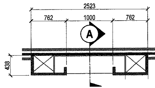
BLOW - UP PLAN
