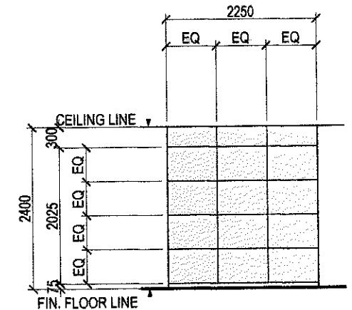
ELEVATION "E"
