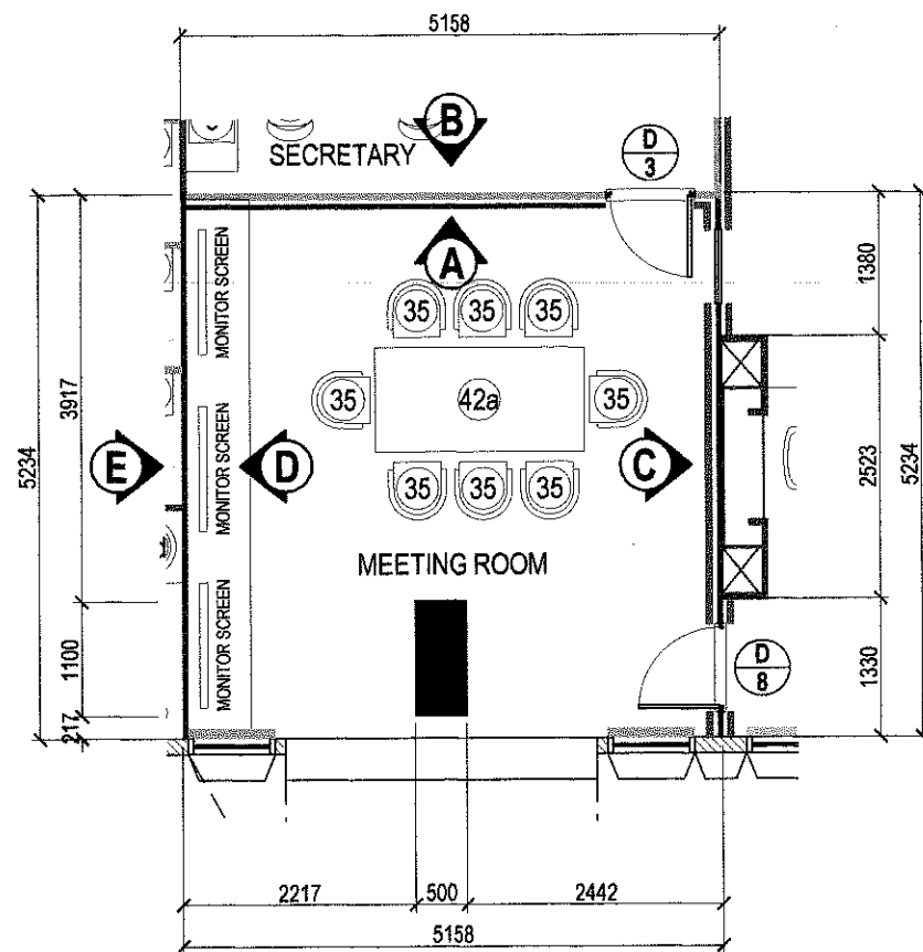
BLOW - UP PLAN
