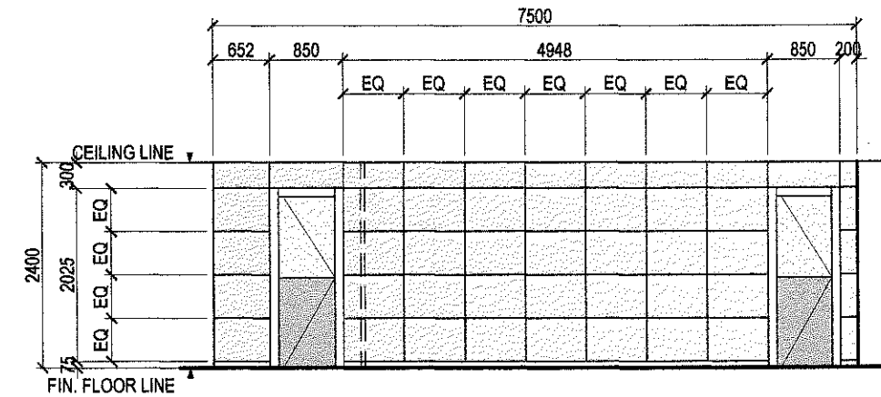
ELEVATION 'A'
