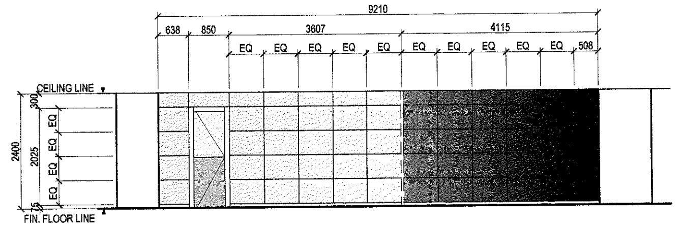
ELEVATION "F"
