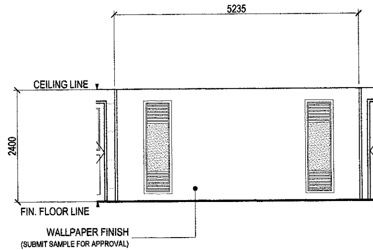
ELEVATION 'A'
