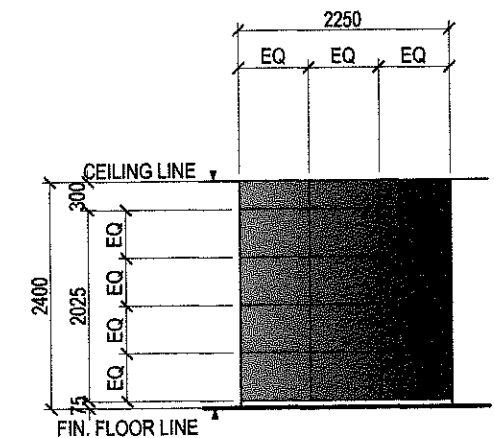
ELEVATION "F"
