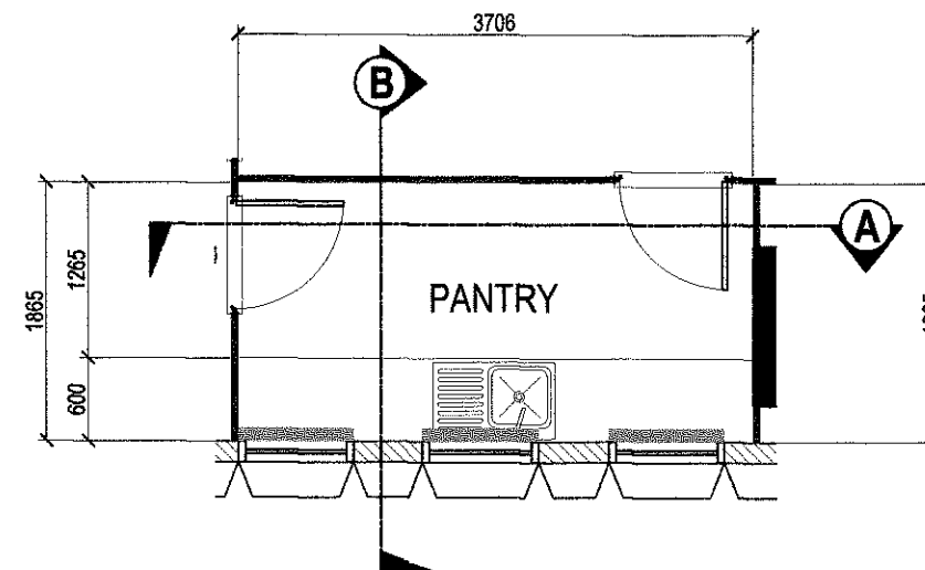
BLOW - UP PLAN
