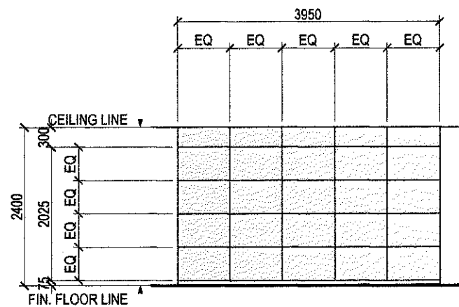
ELEVATION 'A'
