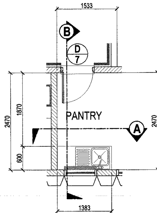
BLOW - UP PLAN
