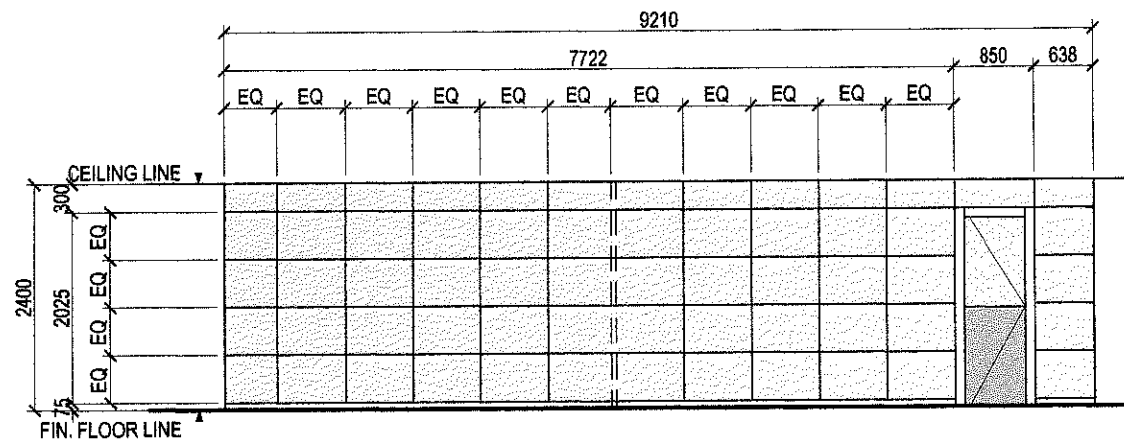
ELEVATION "E"
