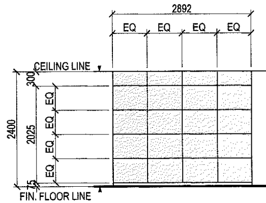
ELEVATION 'A'
