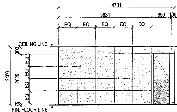
ELEVATION 'A'
