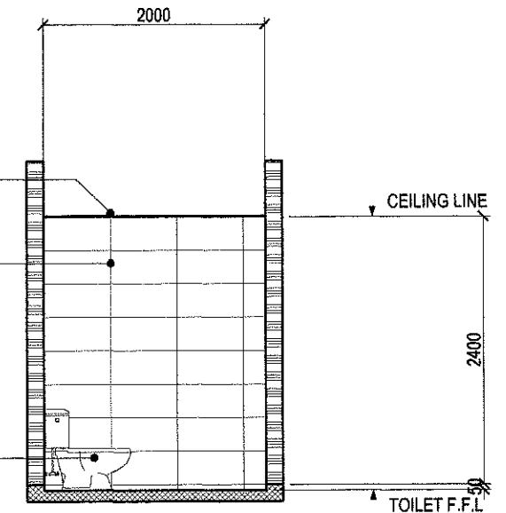
SECTION THRU 'C'
