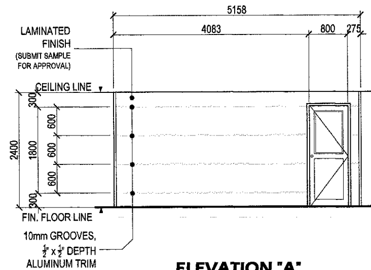
ELEVATION "A"
