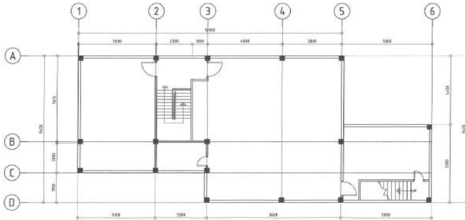
SECOND FLOOR
