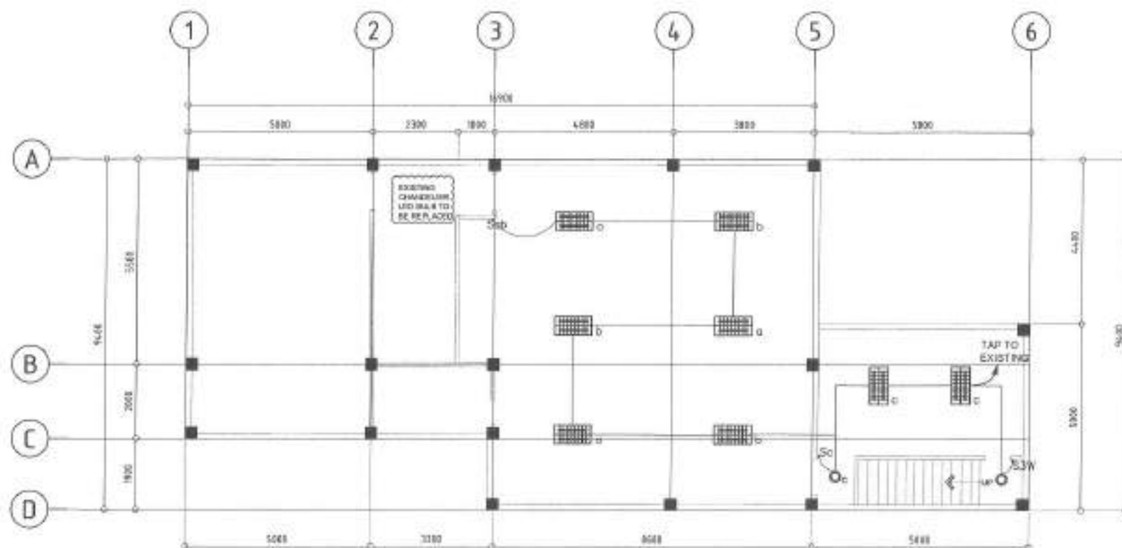
SECOND FLOOR
