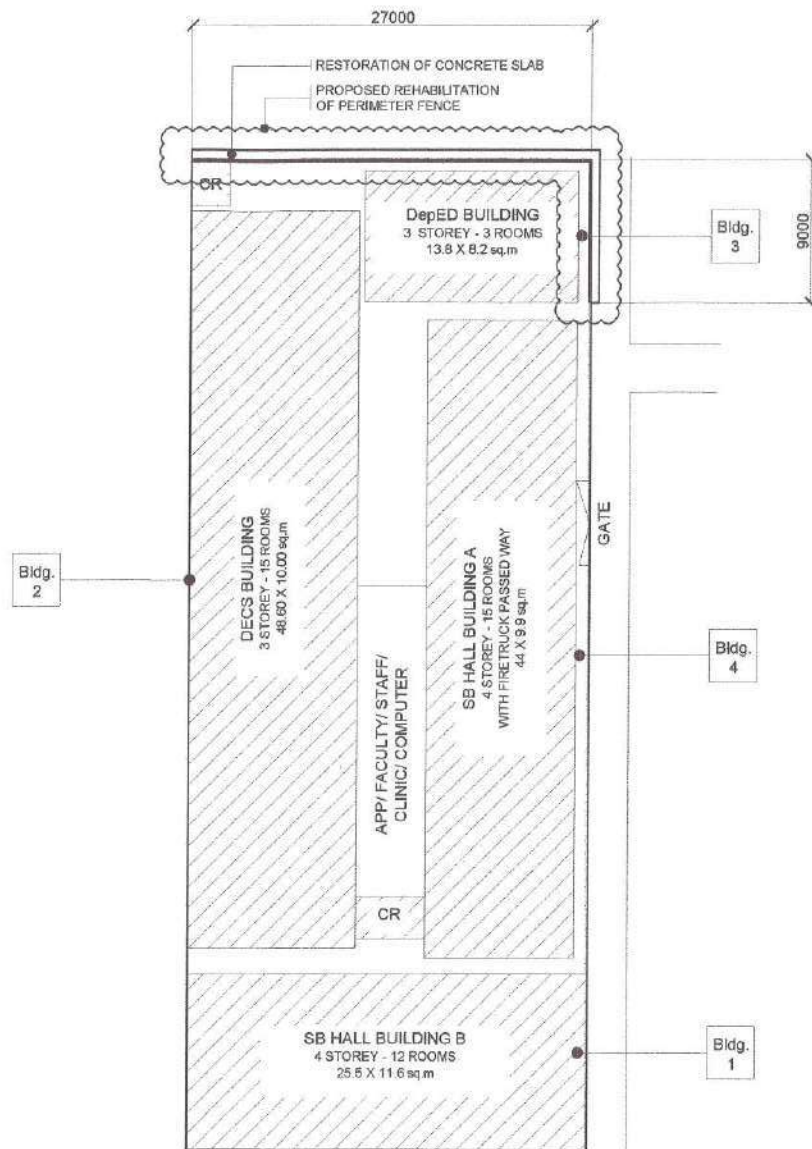
3 SITE DEVELOPMENT PLAN
