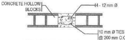
STIFFENER COLUMN DETAIL
