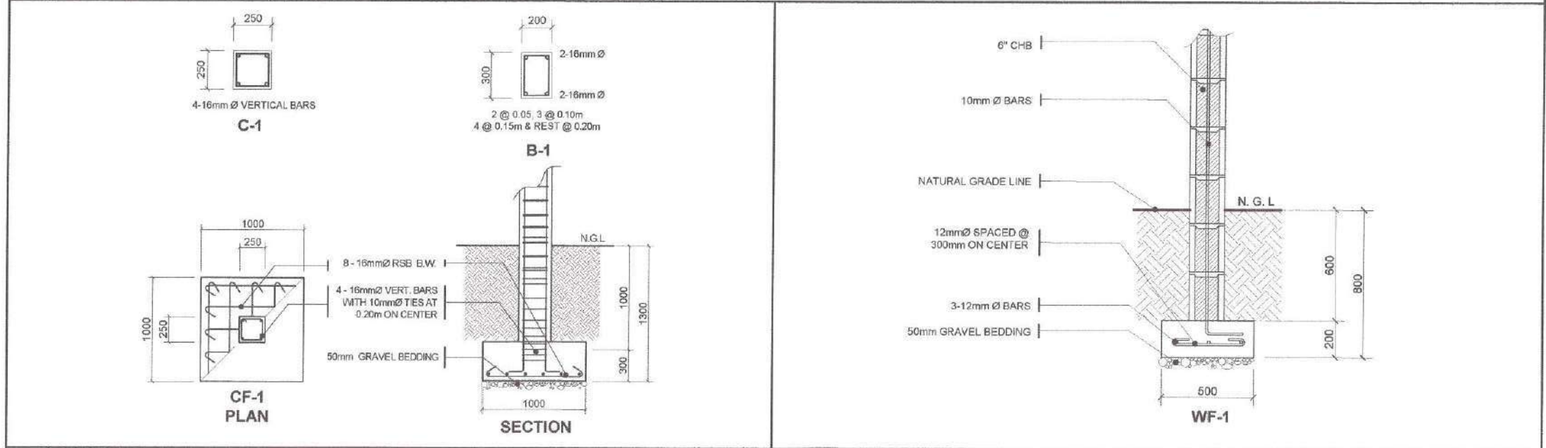
2 DETAILS OF COLUMN, FOOTING AND BEAM SCALE : N.T.S. 3 WALL FOOTING DETAIL SCALE : N.T.S.
