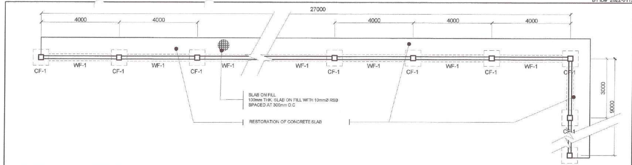
1 FOUNDATION PLAN SCALE : 1:80 METERS
