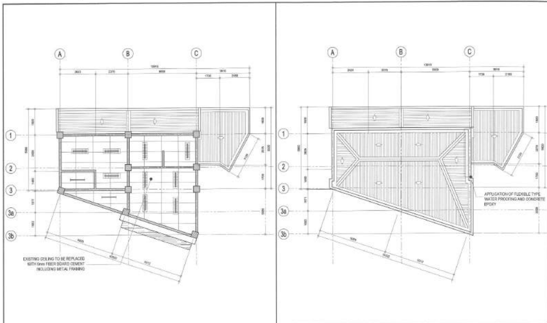
1 SECOND FLOOR REFLECTED CEILING PLAN
