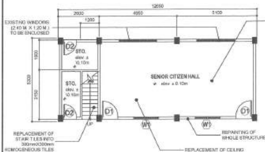
3 PROPOSED GROUND FLOOR PLAN
