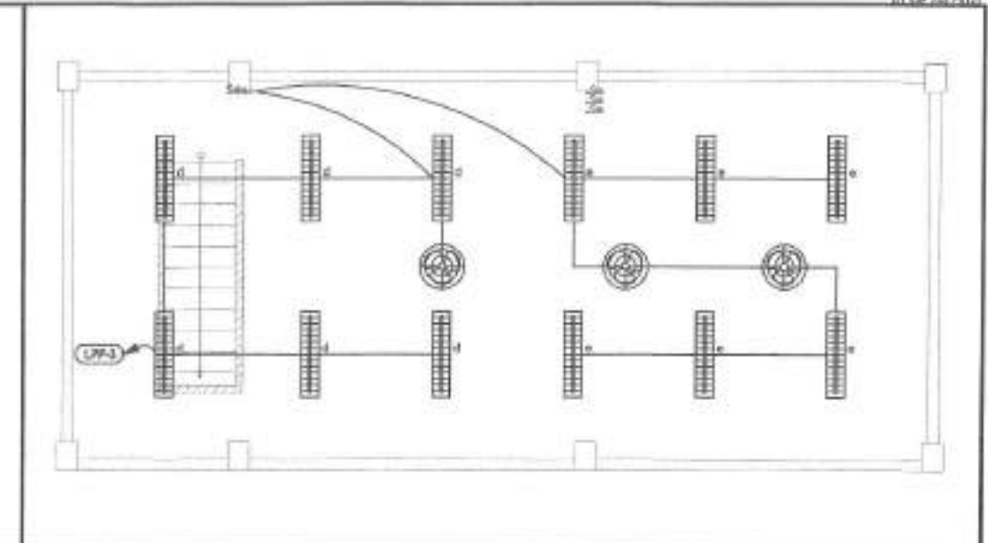
2 SECOND FLOOR LIGHTING LAYOUT
