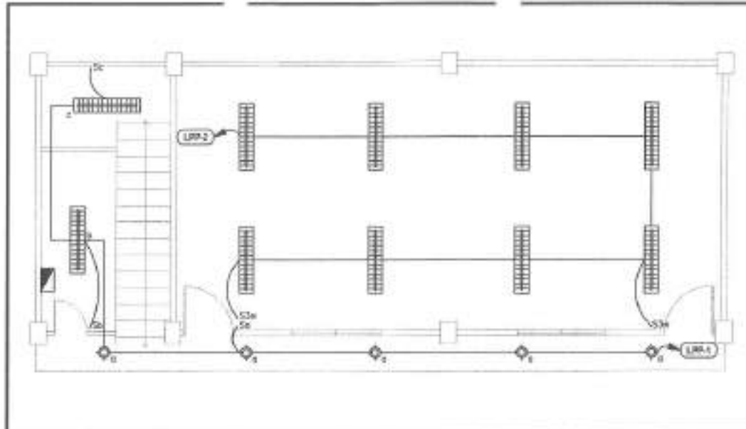
1 GROUND FLOOR LIGHTING LAYOUT
