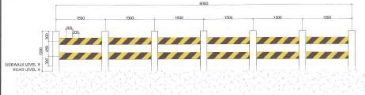
CONCRETE RAILING DETAIL
