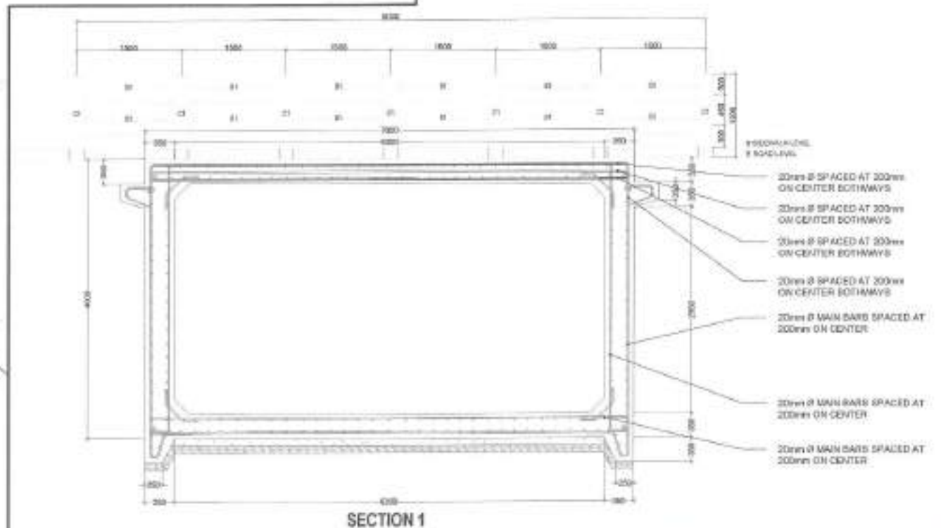
1 BOX CULVERT PLAN (SPL47i) SCALE: NTS 2 BOX CULVERT SECTION (SPL47i) SCALE: NTS
