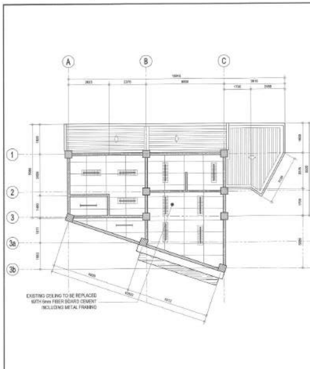
1 SECOND FLOOR REFLECTED CEILING PLAN
