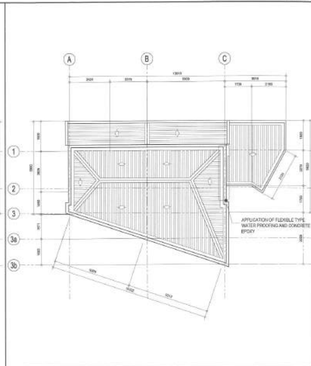
2 ROOF PLAN
