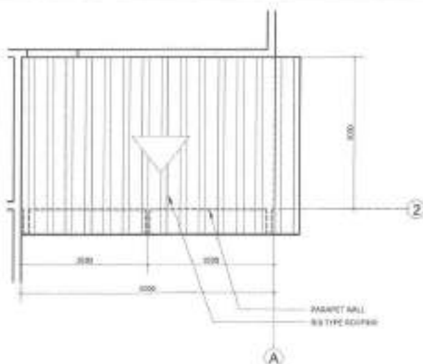
2 TERRACE ROOFING PLAN
