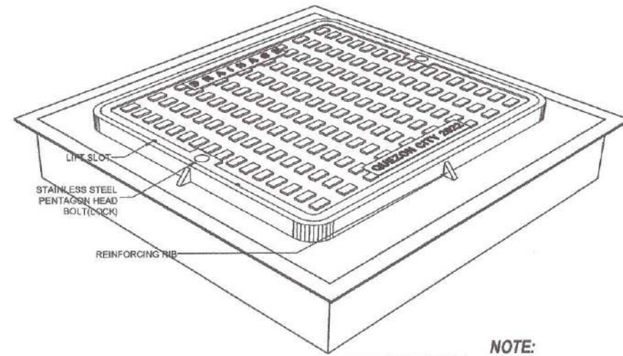
ISOMETRIC VIEW
