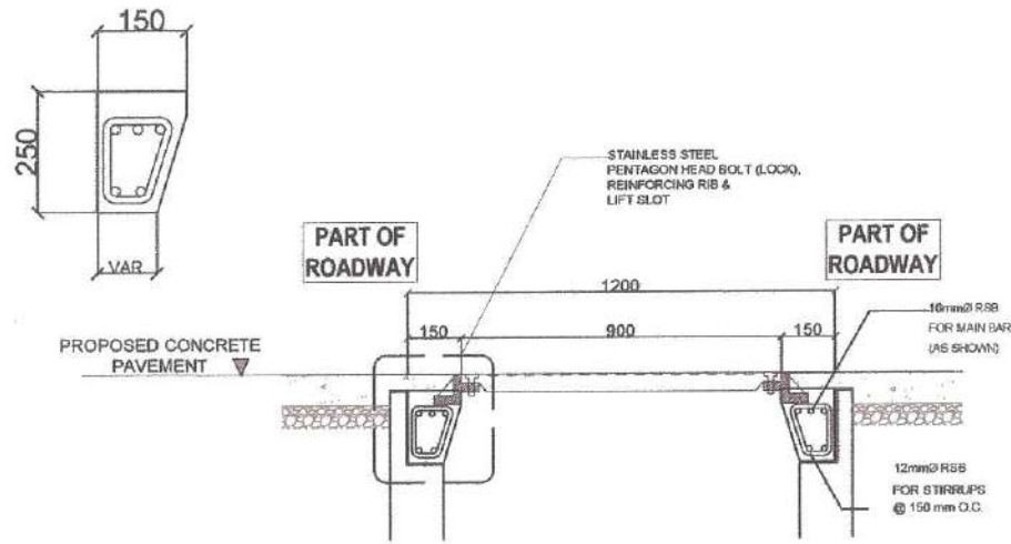
ELEVATION SECTION
