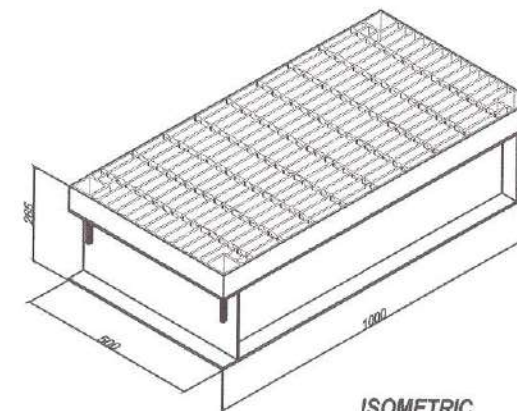
ISOMETRIC
