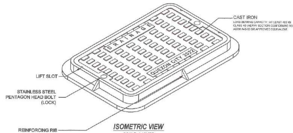
IRON CAST COVER DETAIL SCALE: 1:10MTS
