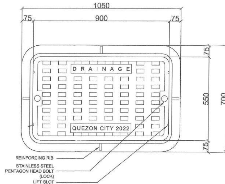
IRON CAST COVER DETAIL SCALE: 1:10MTS
