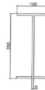
I BEAM DETAIL
