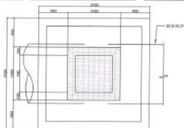
INTERCEPTOR PLAN
