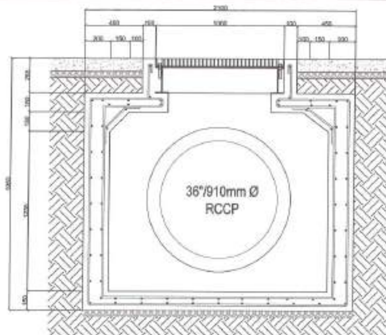
ELEVATION SECTION
