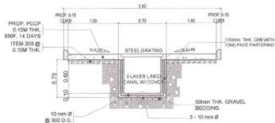
3 ROADWAY SECTION OF D
