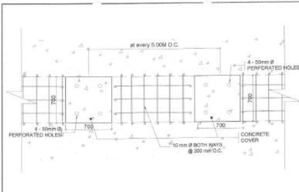
1 2 LAYER & 3 LAYER LINED CANAL CONCRETE COVER DETAIL
