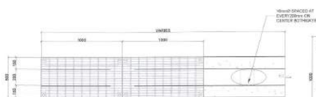
INTERCEPTOR PLAN SCALE: 1:20MTS
