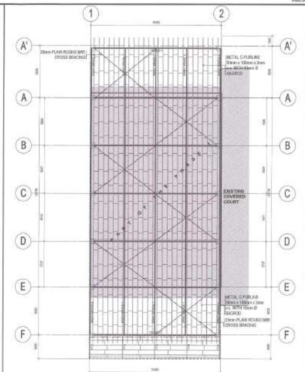
2 ROOF FRAMING PLAN
