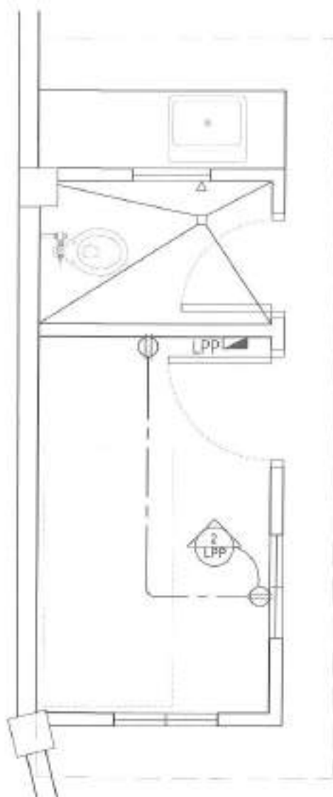
1 GF POWER LAYOUT E-2 SCALE 1:30
