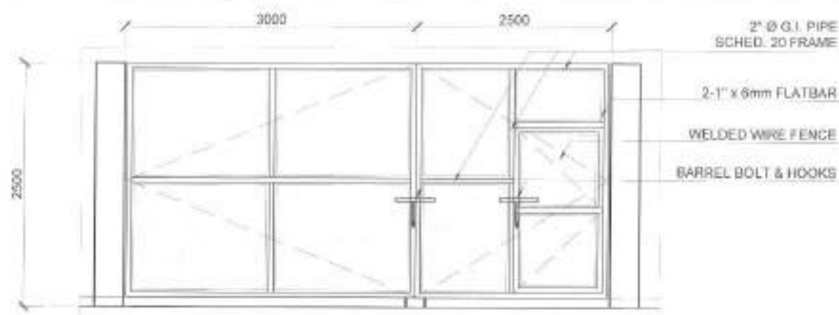
4 GATE 1 DETAIL A4 SCALE 1:40
