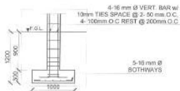
3 COLUMN FTG. DETAIL A4 SCALE 1/40
