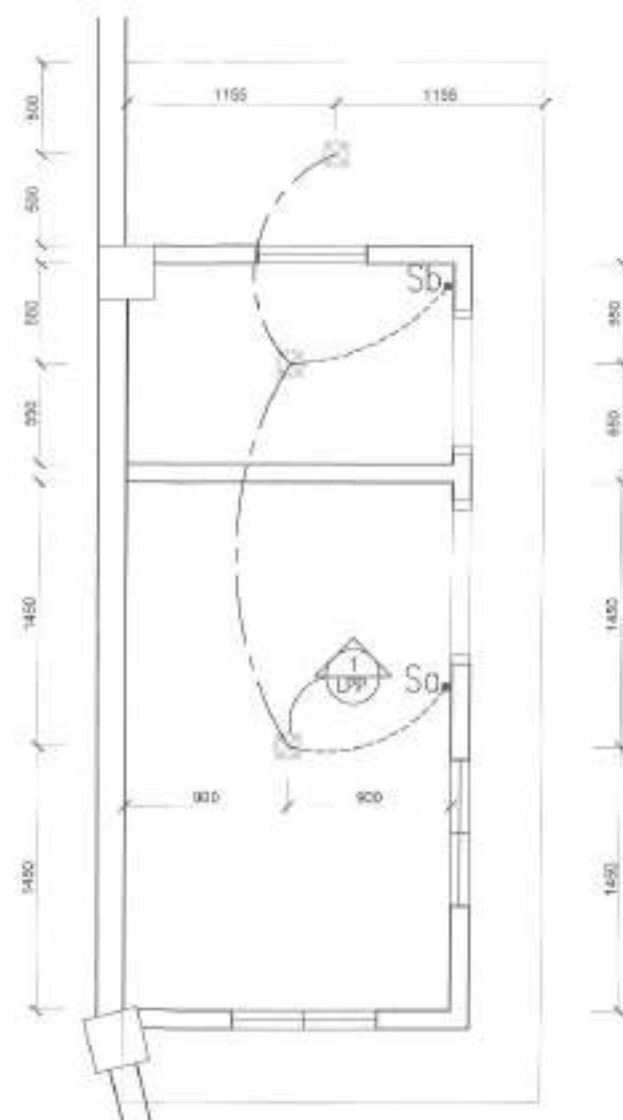
2 GF LIGHTING LAYOUT E-2 SCALE 1:30
