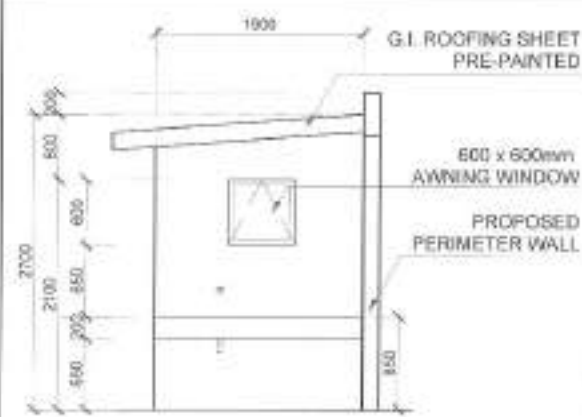
2 FRONT ELEVATION A3 SCALE 1:50
