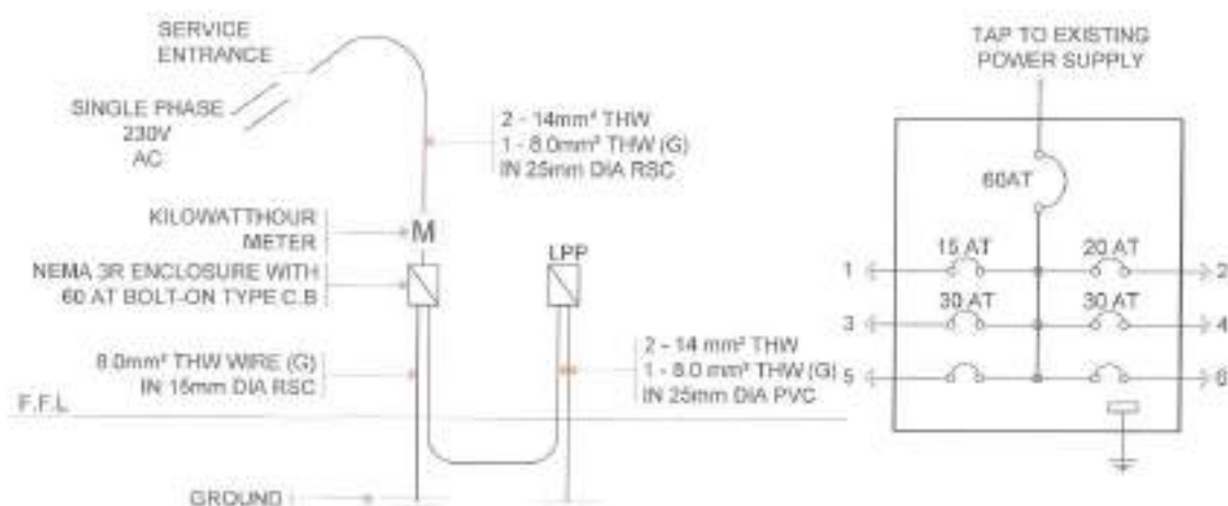
3 POWER RISER DIAGRAM E-1 SCALE NTS
