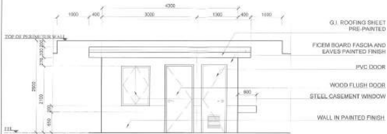
2 FRONT ELEVATION A3 SCALE 1:50
