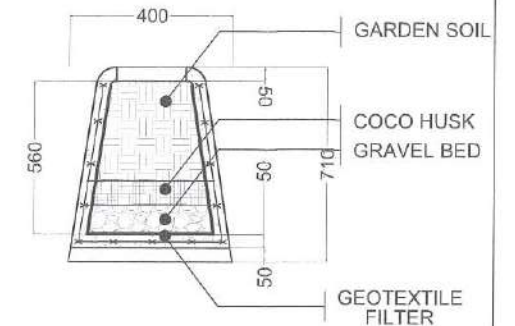
D SECTIONS 03 SCALE 1:20
