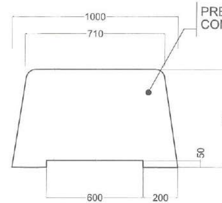
C FRONT ELEVATION 03 SCALE 1:20
