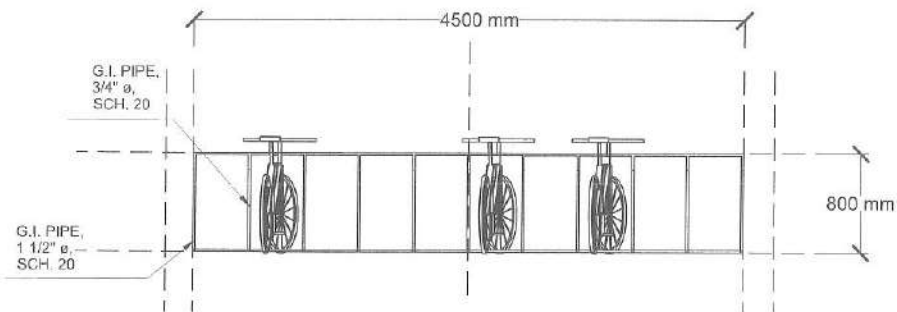
B FRONT ELEVATION 01 SCALE 1:30
