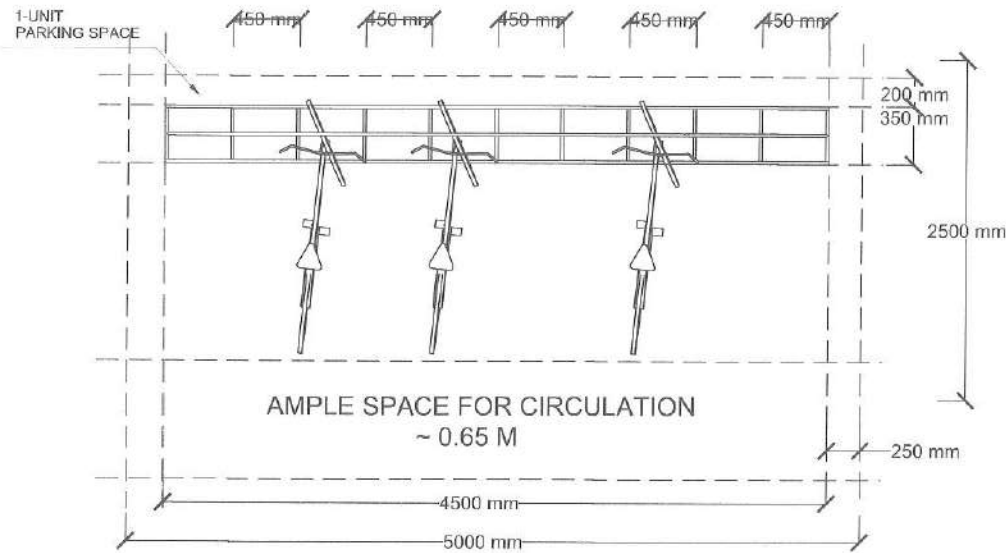
A PLAN VIEW 01 SCALE 1:30
