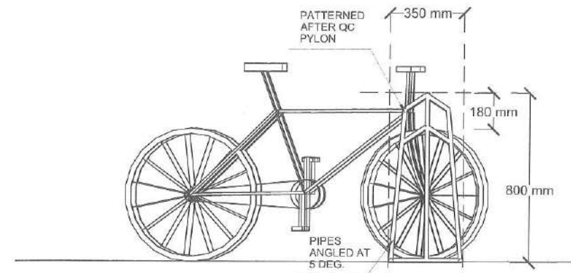
C SIDE ELEVATION 01 SCALE 1:30
