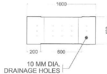
B BOTTOM VIEW 03 SCALE 1:20
