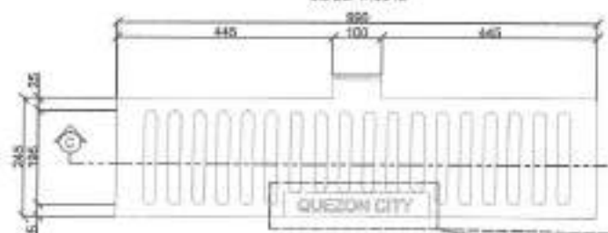
COVER WITH PERFORATED HOLES SCALE: 1:10MTS
