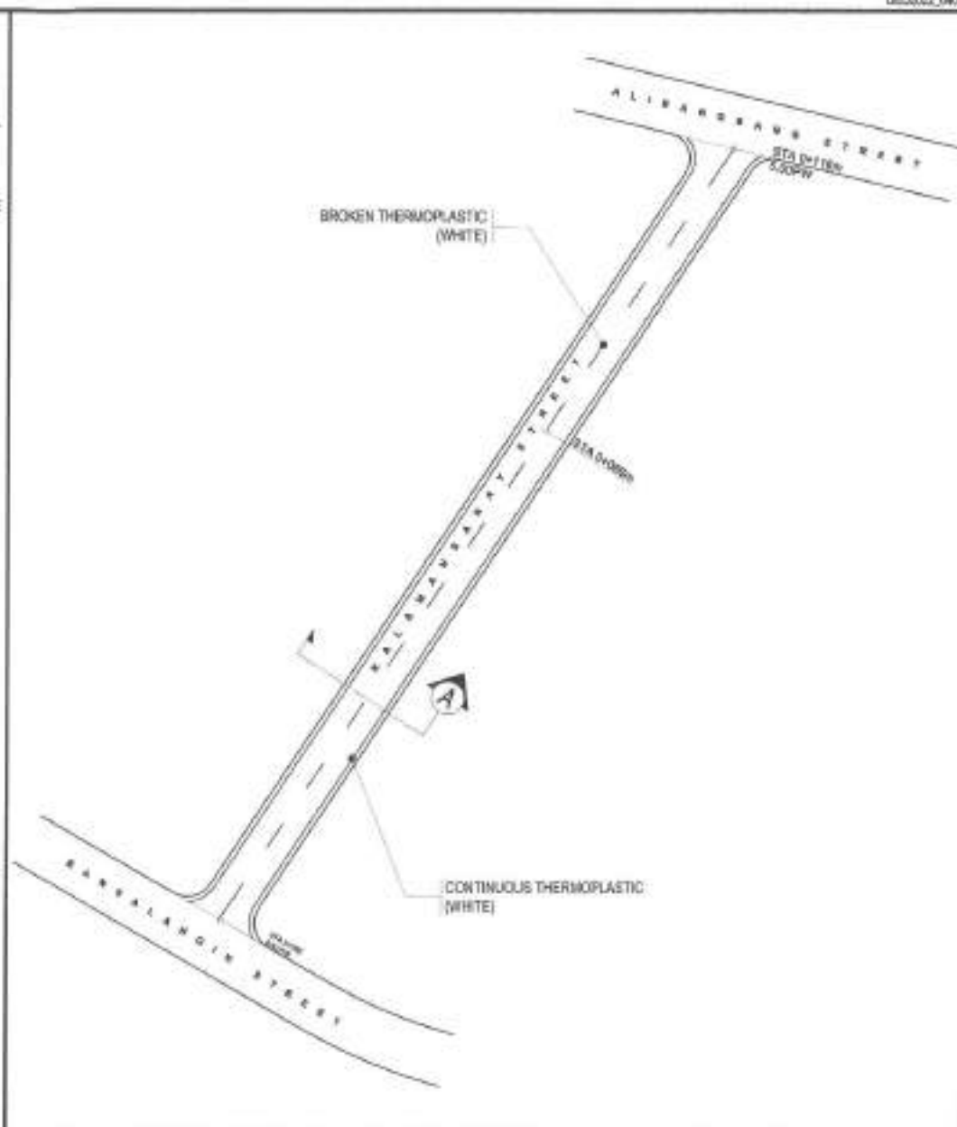
2 ROADWAY PLAN WITH THERMOPLASTIC LANE MARKINGS
