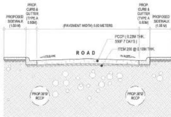
1 ROAD CROSS SECTION OF A
