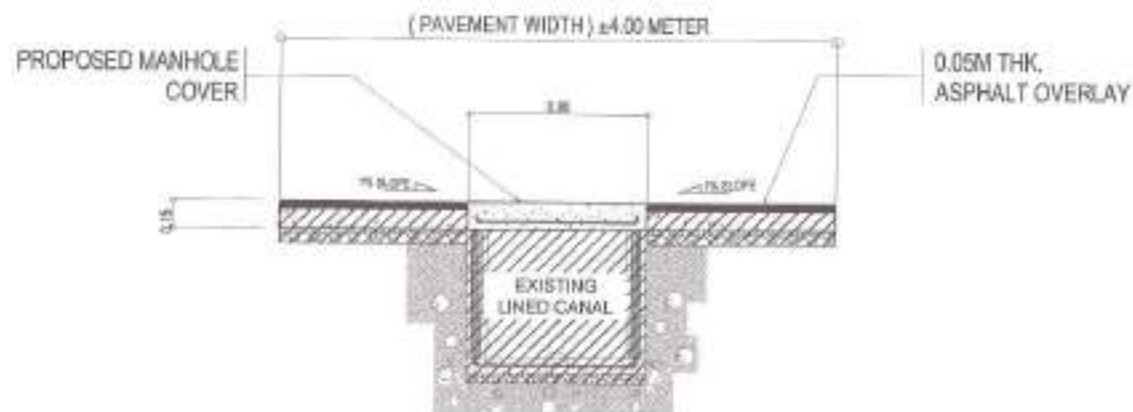
2 TYPICAL DETAIL FOR 3-LAYER LINED CANAL
