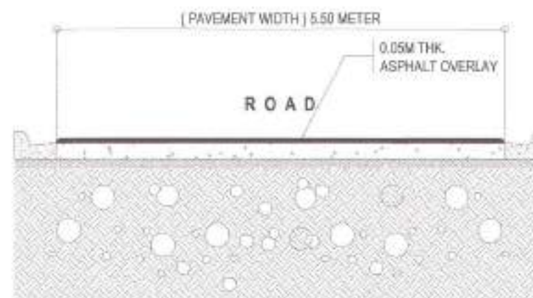
2 ROADWAY CROSS SECTION OF B
