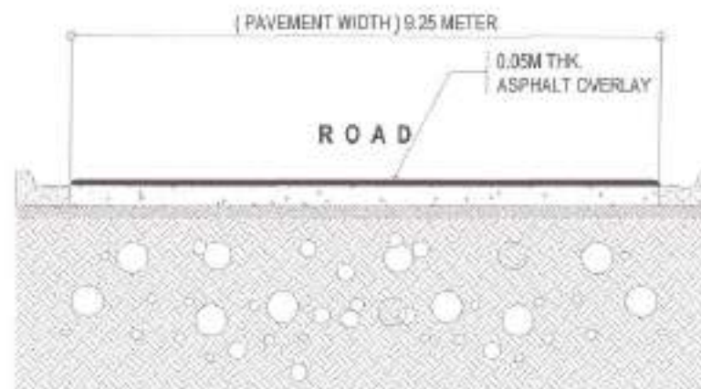
4 ROADWAY CROSS SECTION OF D
