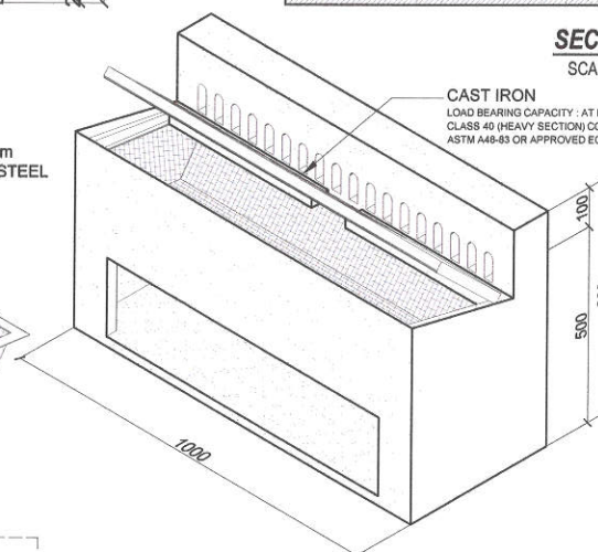
ISOMETRIC SCALE: 1:15MTS
