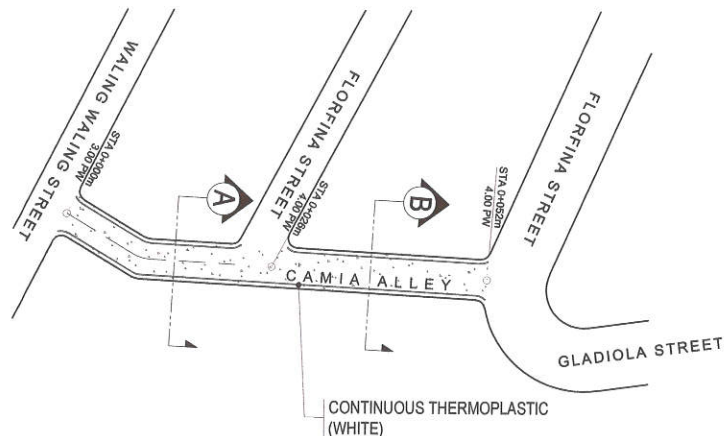
1 ROADWAY PLAN
