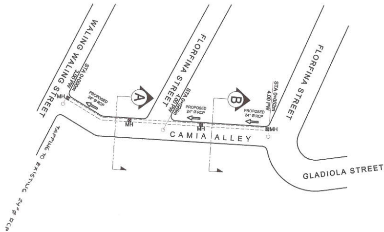
1 ROADWAY PLAN
