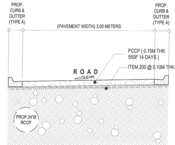
3 ROAD CROSS SECTION OF A
