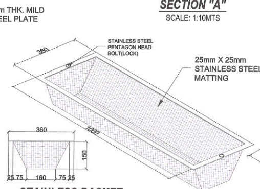
STAINLESS BASKET SCALE: 1:15MTS
