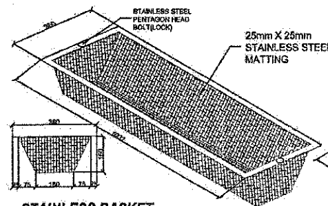
STAINLESS BASKET SCALE: 1:15MTS
