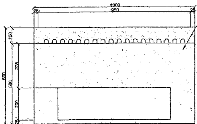
FRONT VIEW SCALE: 1:10MTS
