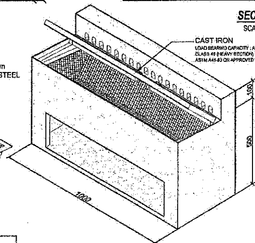
ISOMETRIC SCALE: 1:15MTS
