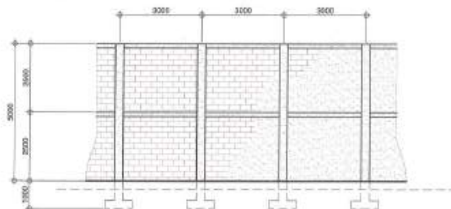
3 ELEVATION (CHB FENCE)
