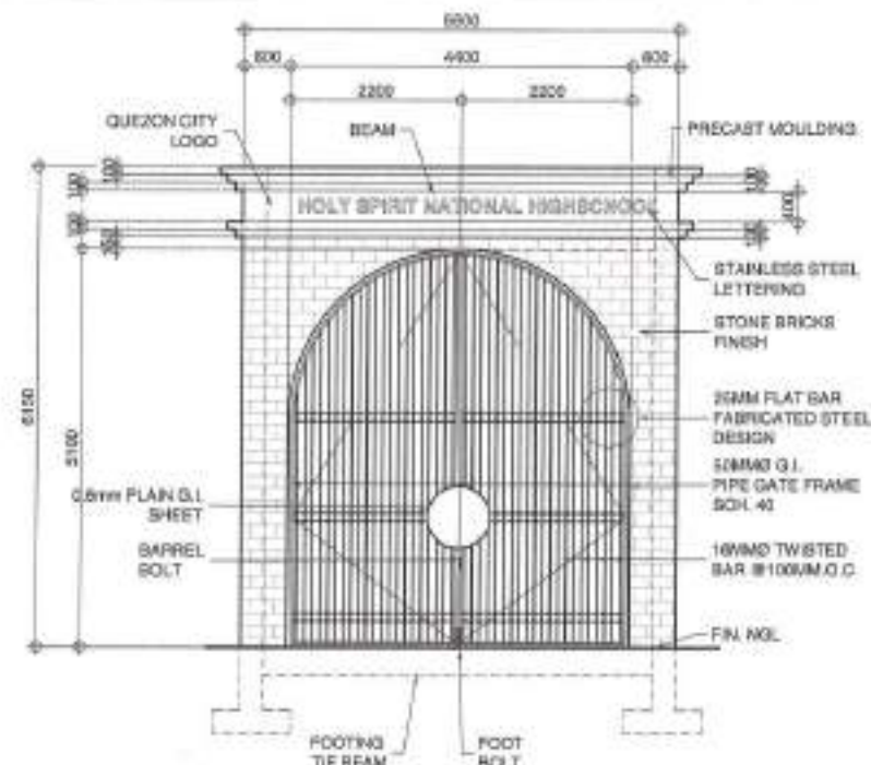
2 STEEL GATE DETAILS
