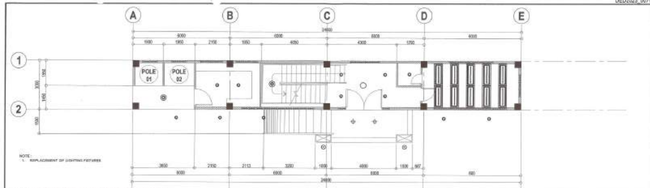
1 GROUND FLOOR LIGHTING LAYOUT
