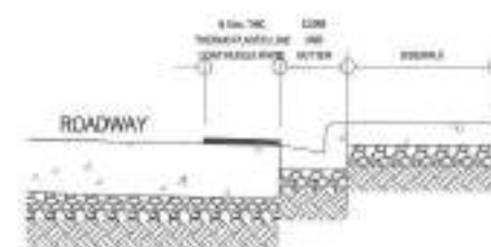
THERMO PLASTIC CROSS SECTION
