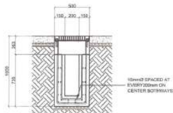
ELEVATION SECTION
