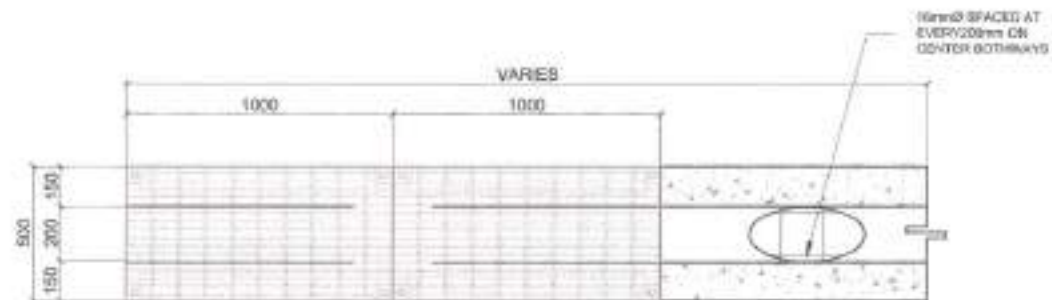
INTERCEPTOR PLAN
