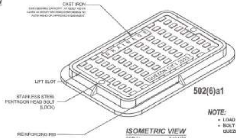
IRON CAST COVER DETAIL SCALE: 1:10MTS
