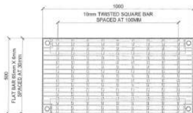
1000mm X 500mm STEEL GRATING MANHOLE
