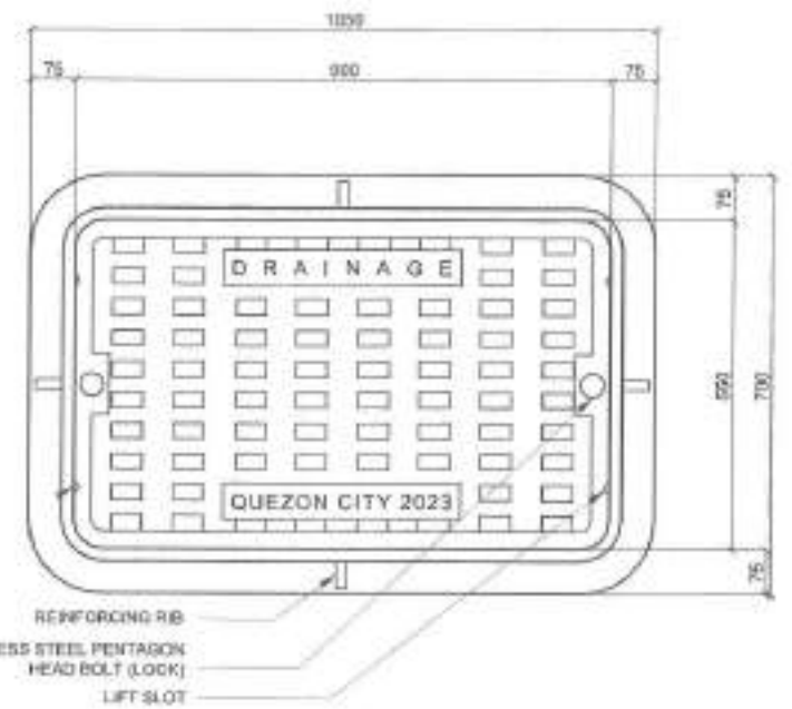
IRON CAST COVER DETAIL SCALE: 1:10MTS
