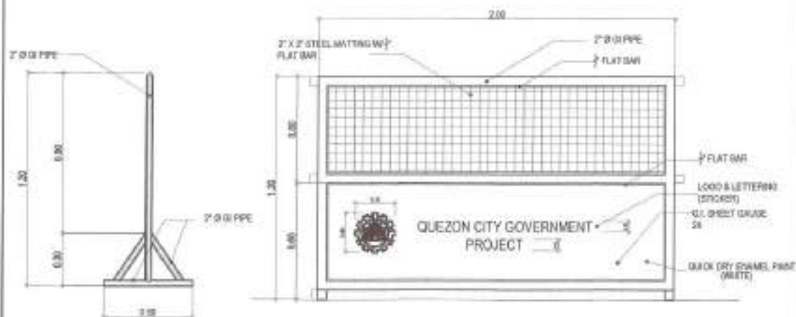
3 ROAD SAFETY BARRIER SYSTEM (STEEL BARRICADE) DETAIL
